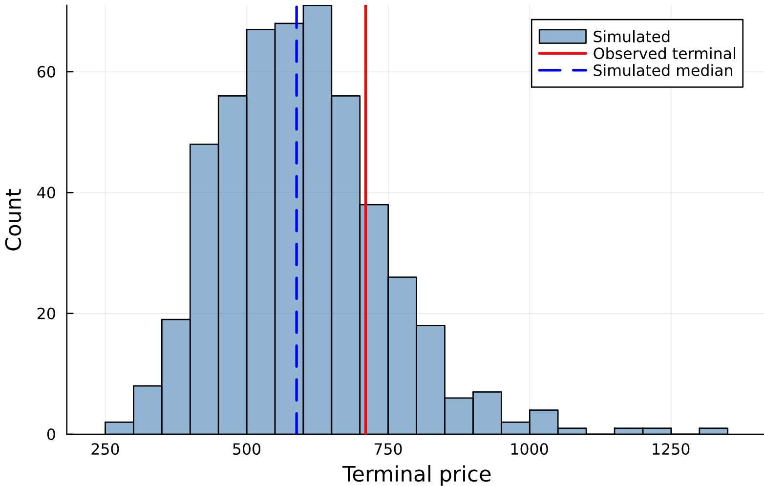
SPY - CHMM-t terminal price (n=500)
