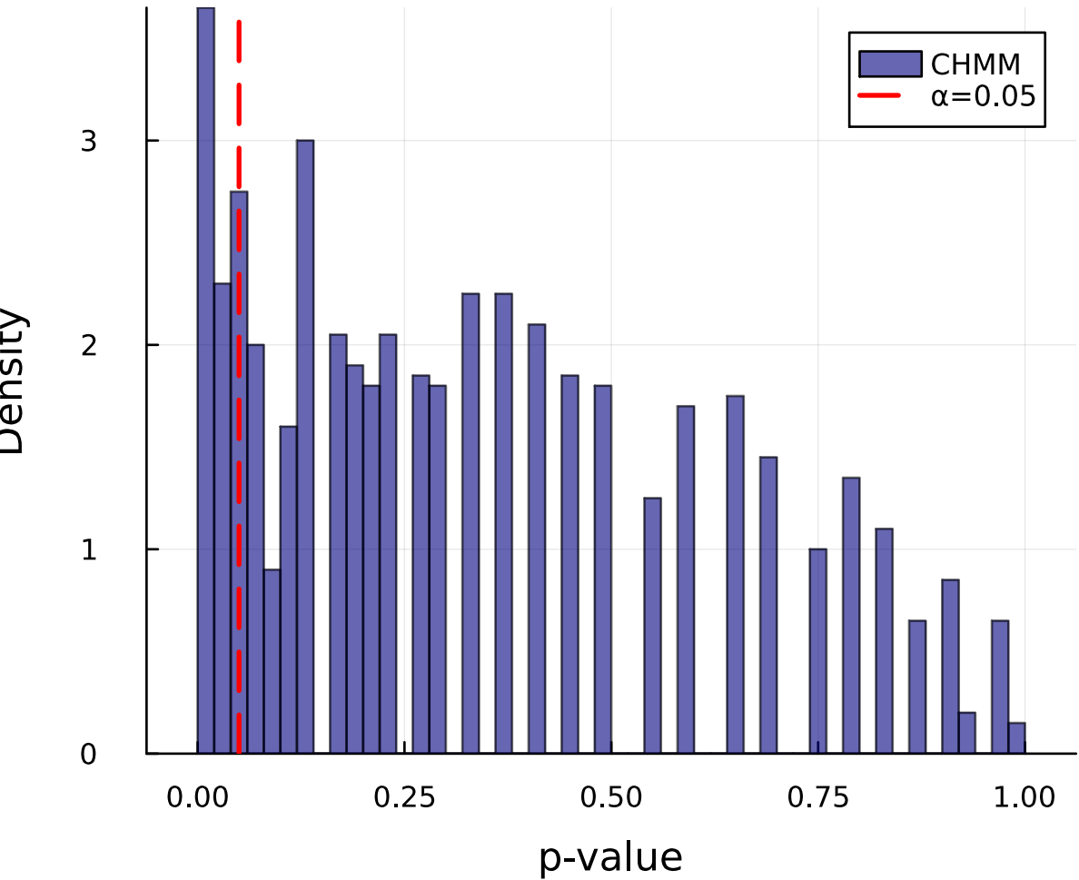
(a) OoS KS p-values
