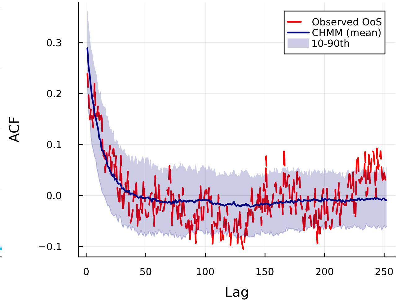
(c) OoS ACF( |G_t| )
