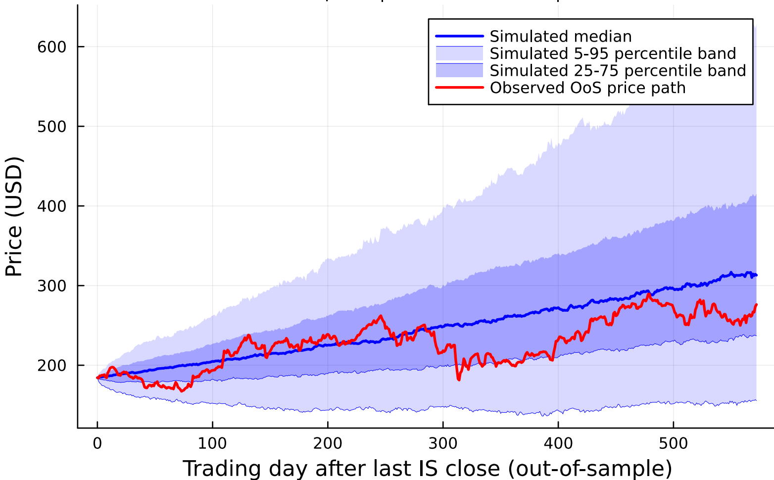
Pipeline A — AAPL OoS price fan | CHMM-N, K=18 500 simulated paths | S0 = last IS VWAP | dt = 1/252
