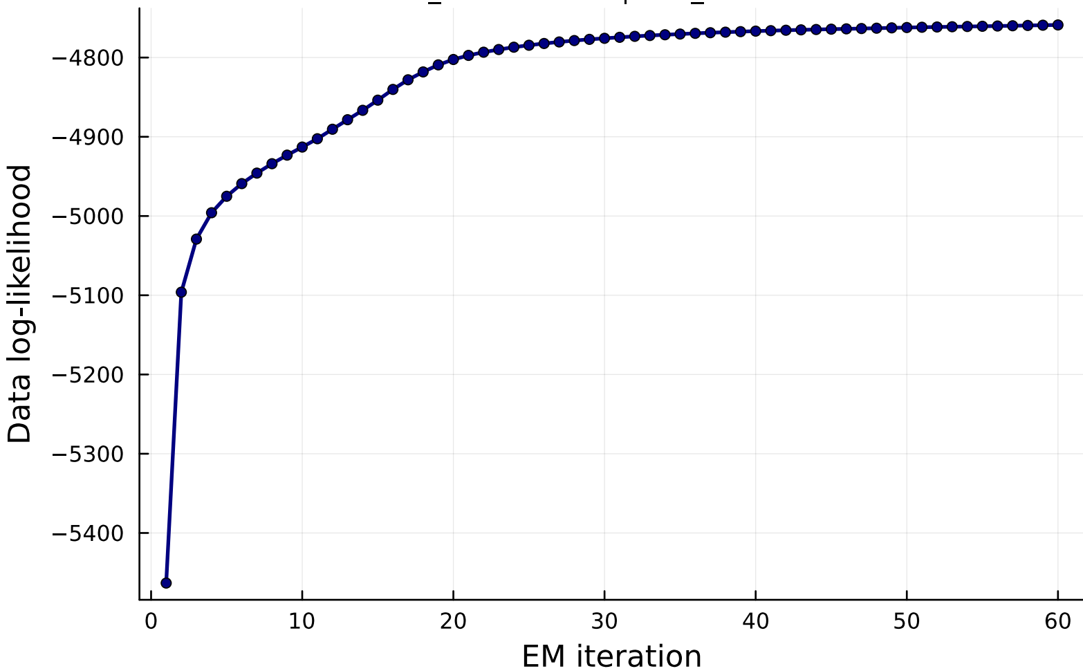
Pipeline A — Baum-Welch convergence | SPY | CHMM-L, K=18 T_IS = 2516 obs | max_iter = 60
