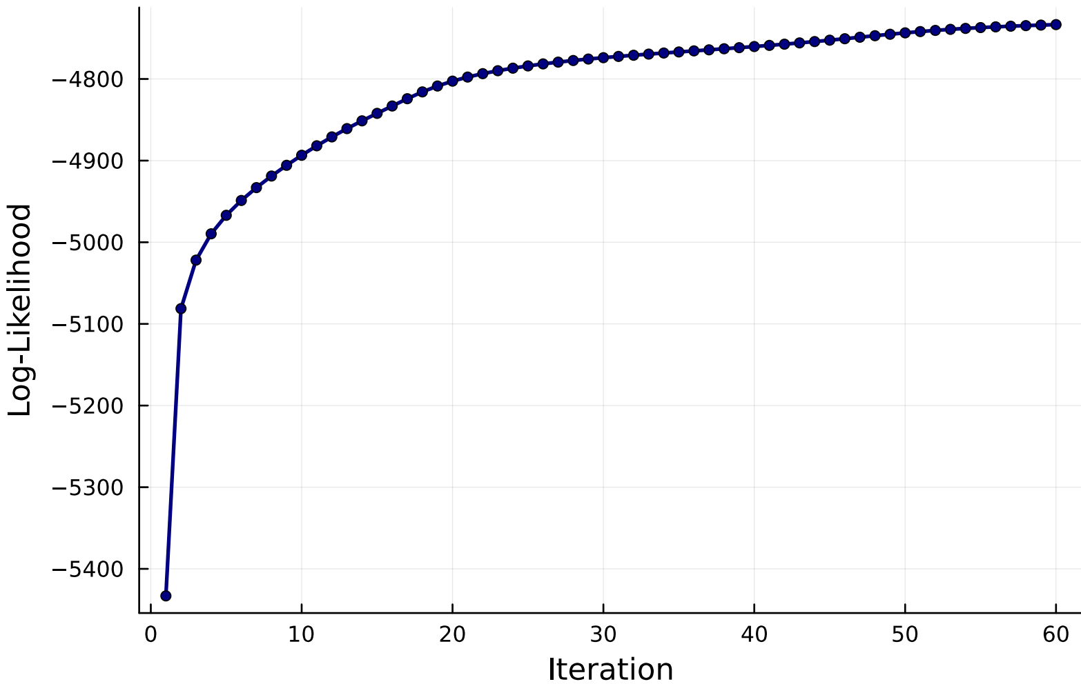
Baum-Welch Convergence (SPY, K=18)
