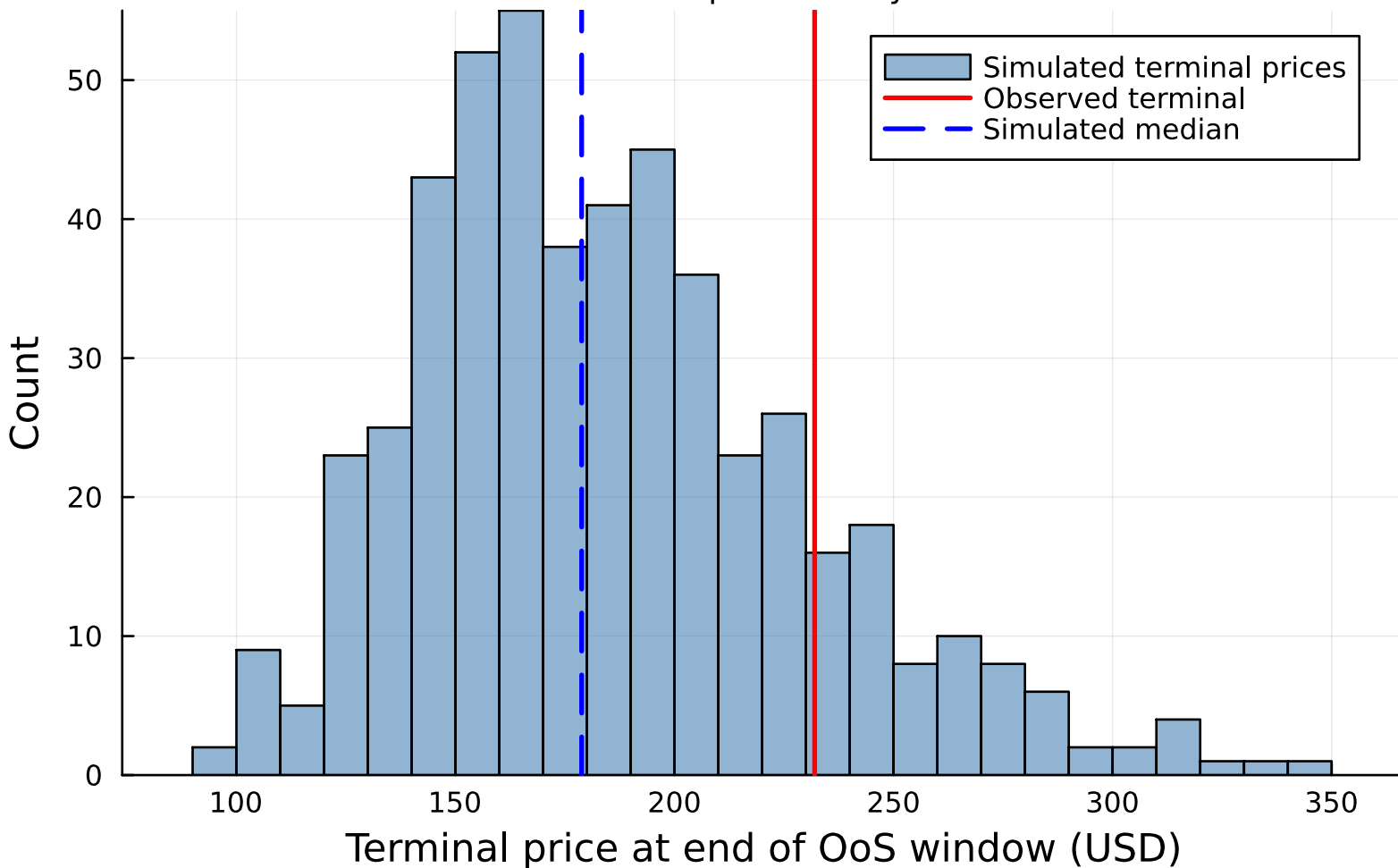
Pipeline A — JNJ terminal-price distribution | CHMM-L, K=18 500 simulated paths at day 572 OoS
