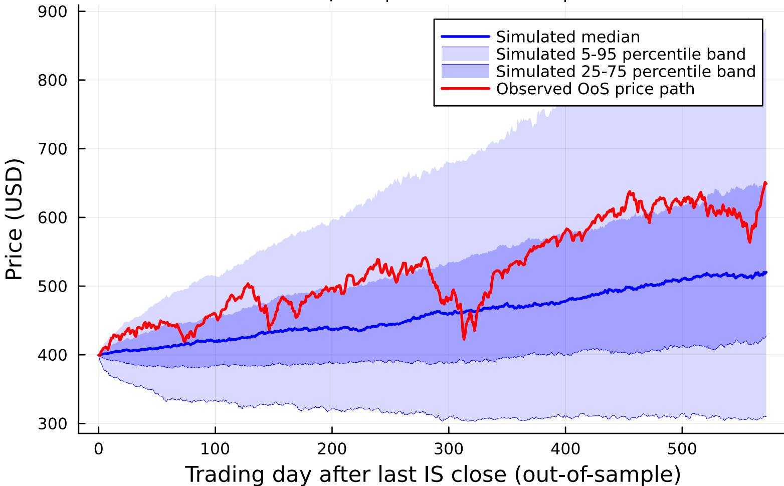
Pipeline A — QQQ OoS price fan | CHMM-L, K=18 500 simulated paths | S0 = last IS VWAP | dt = 1/252
