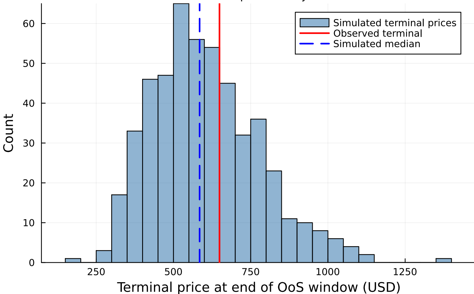
Pipeline A — QQQ terminal-price distribution | CHMM-N, K=18 500 simulated paths at day 572 OoS
