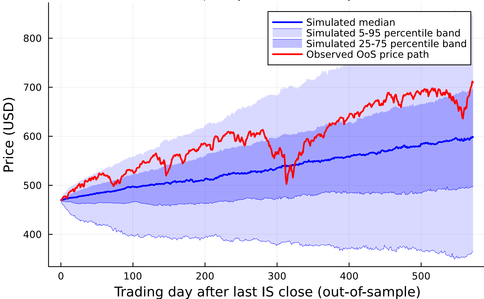
Pipeline A — SPY OoS price fan | CHMM-N, K=18 500 simulated paths | S0 = last IS VWAP | dt = 1/252
