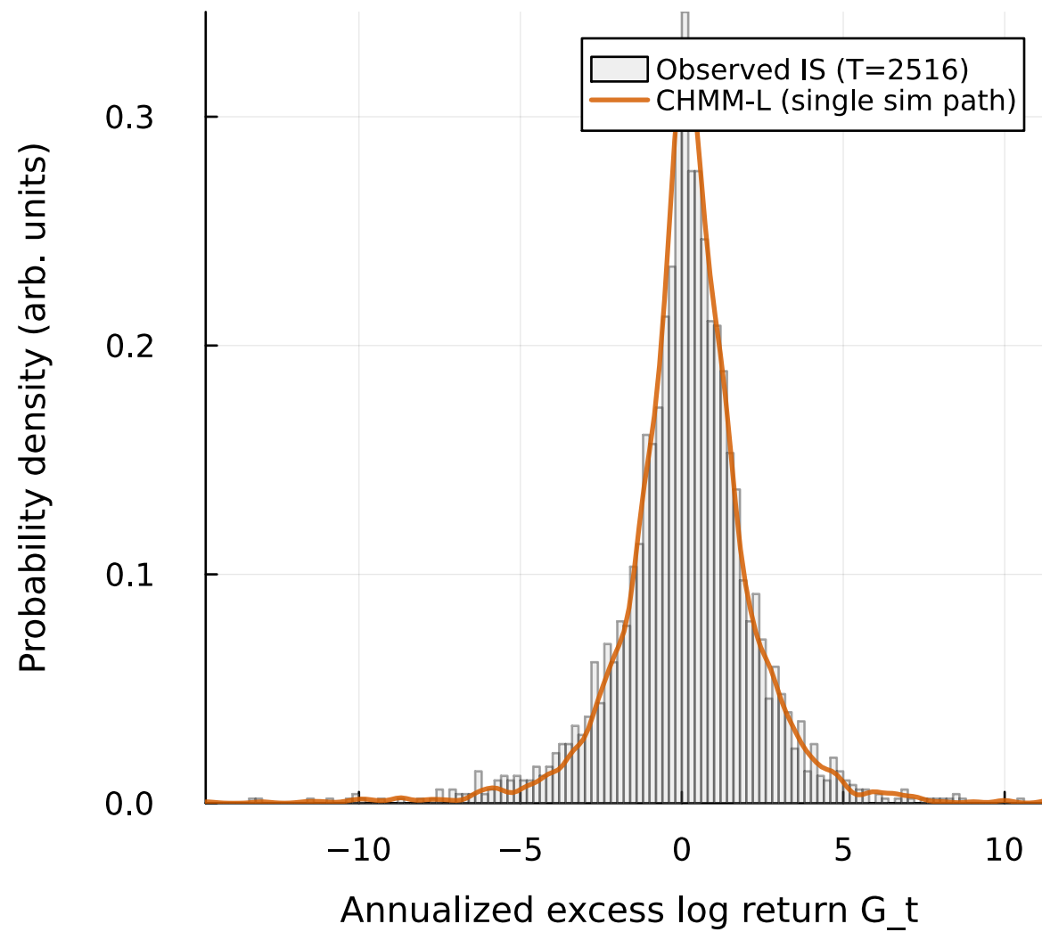
IS return density | KS pass rate = 93.8% of 1000 paths at alpha=0.05
