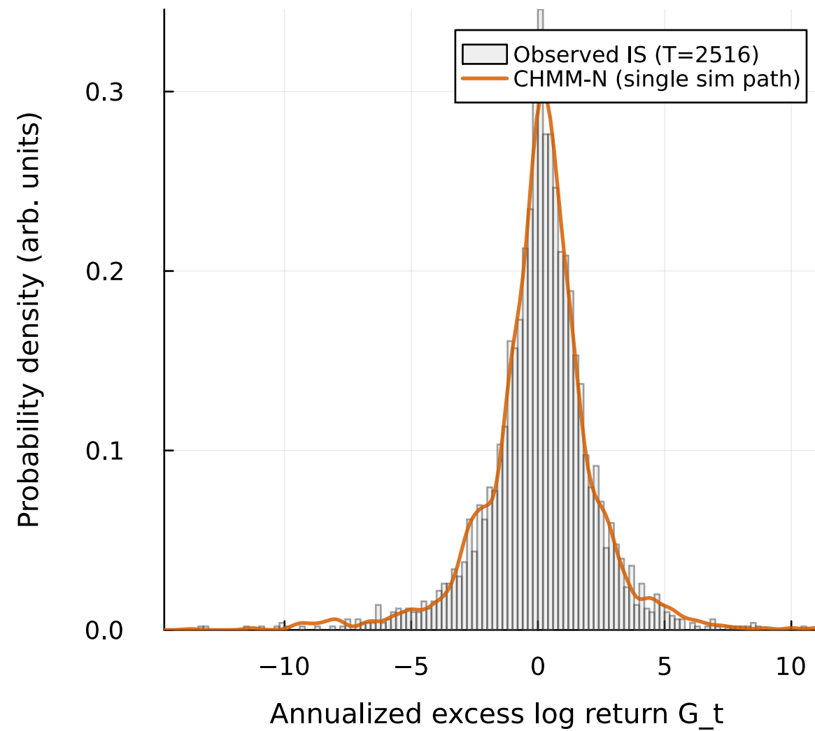
IS return density | KS pass rate = 93.9% of 1000 paths at alpha=0.05
