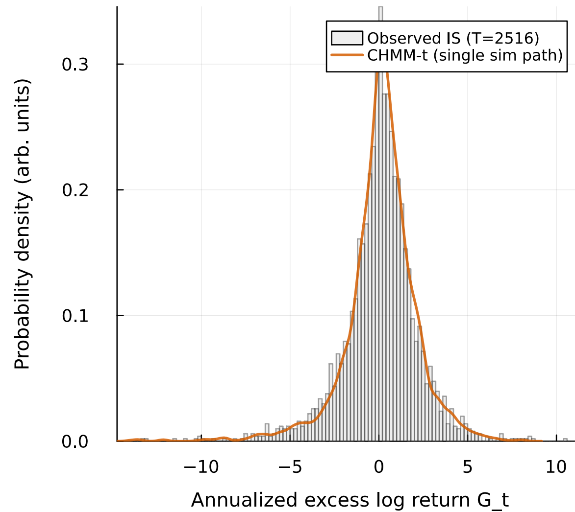
IS return density | KS pass rate = 95.4% of 1000 paths at alpha=0.05
