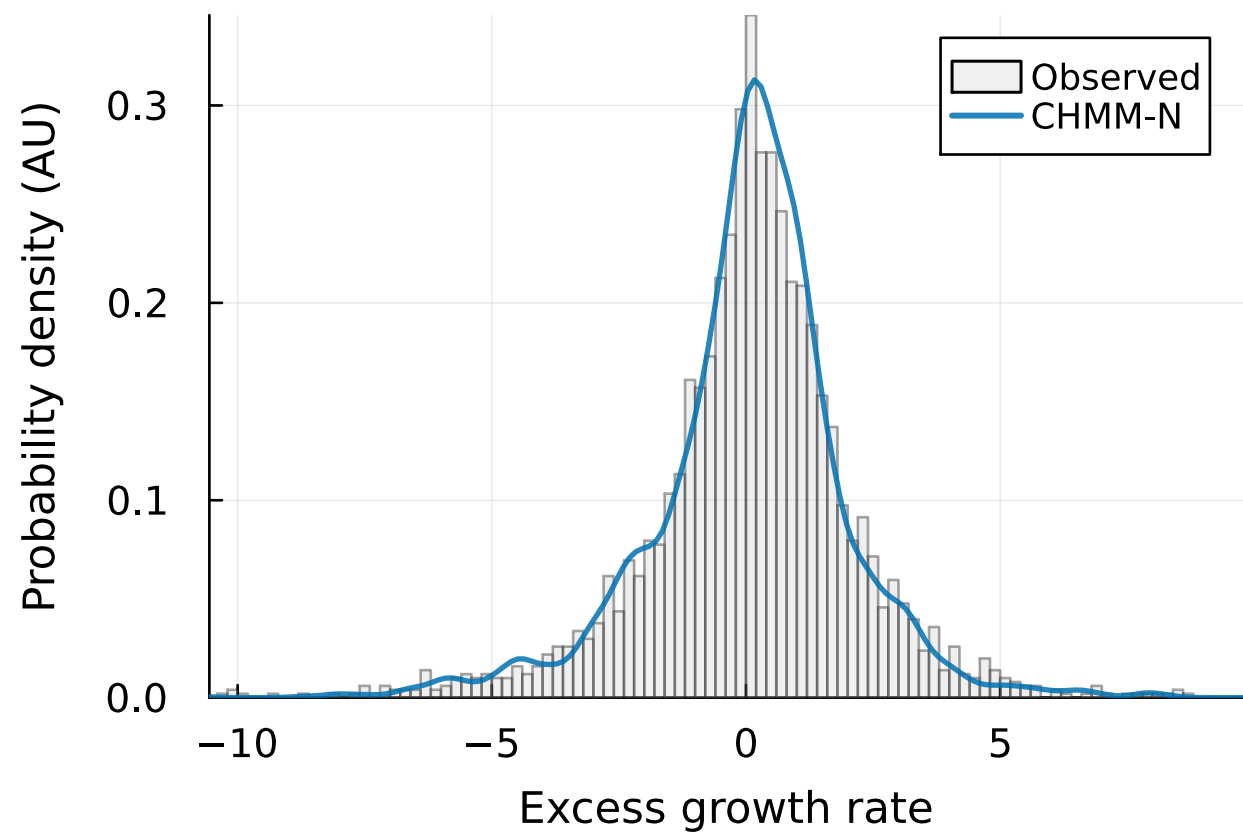
IS density (KS: 94.6%)
