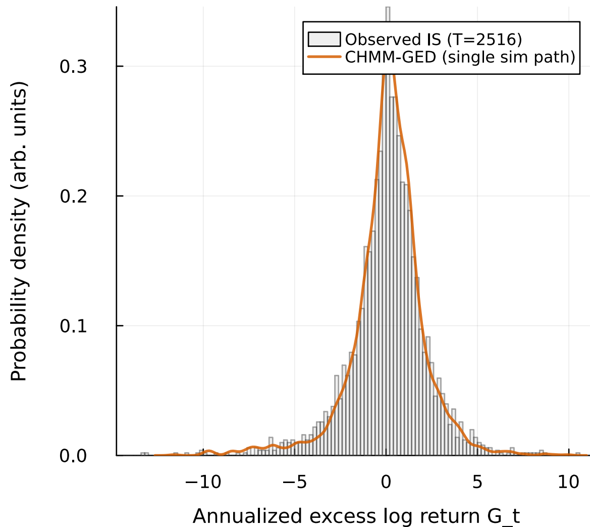
IS return density | KS pass rate = 96.3% of 1000 paths at alpha=0.05
