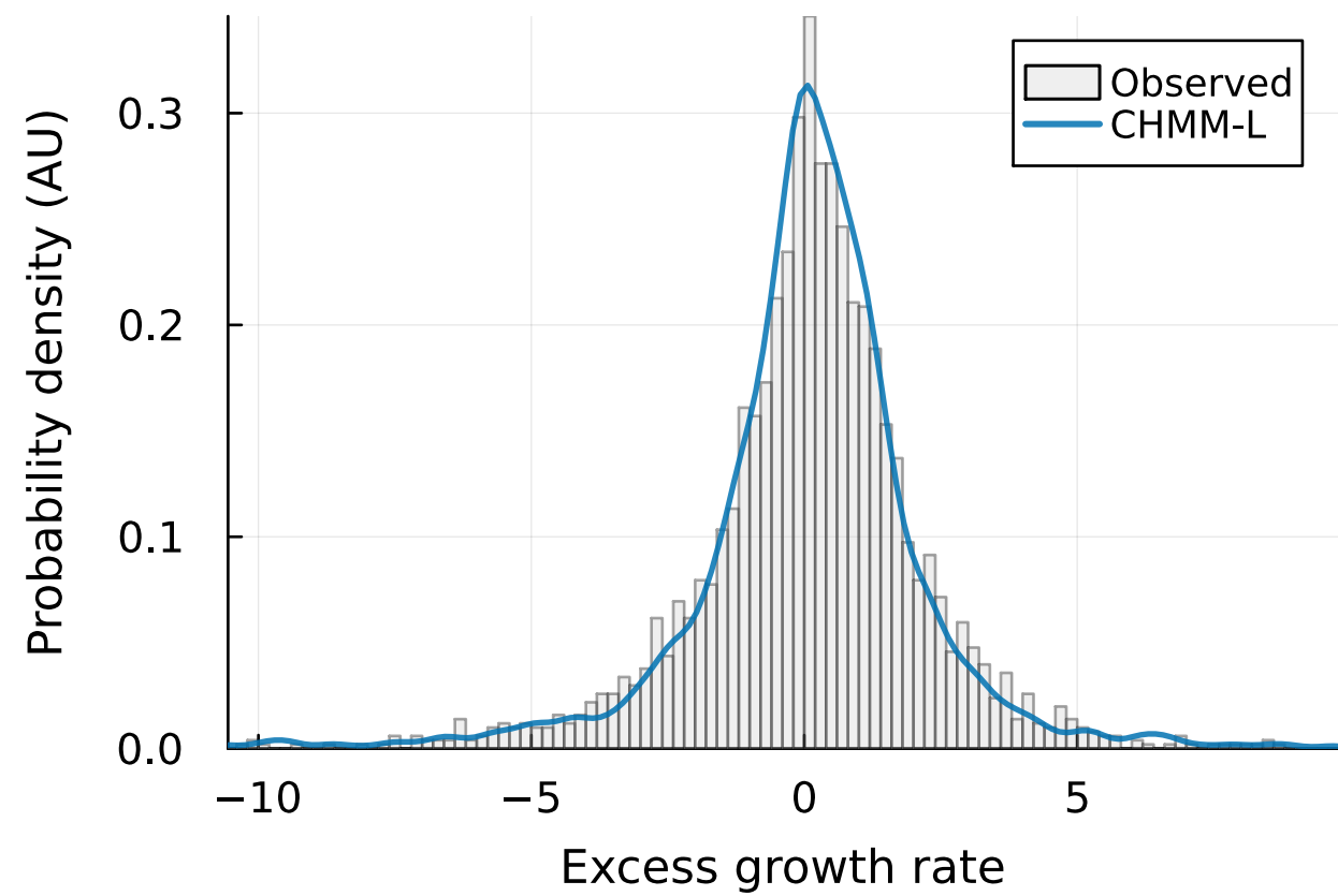
IS density (KS: 95.3%)
