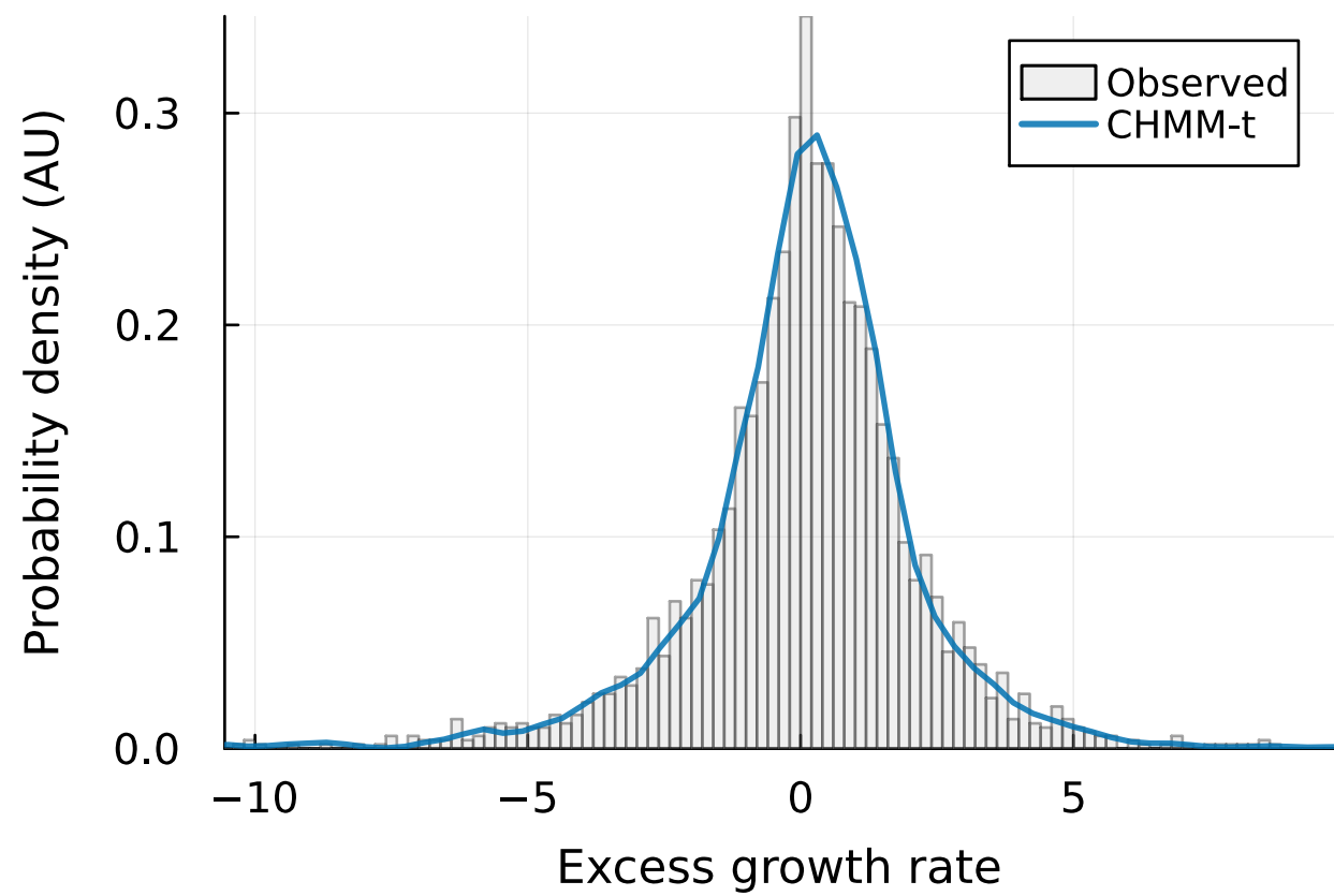
IS density (KS: 95.7%)
