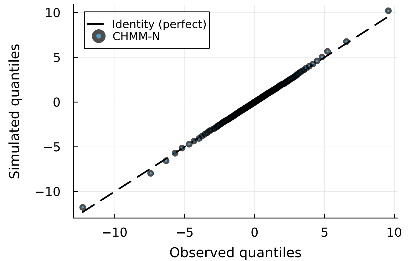
Tail Q-Q plot (0.1st-99.9th)
