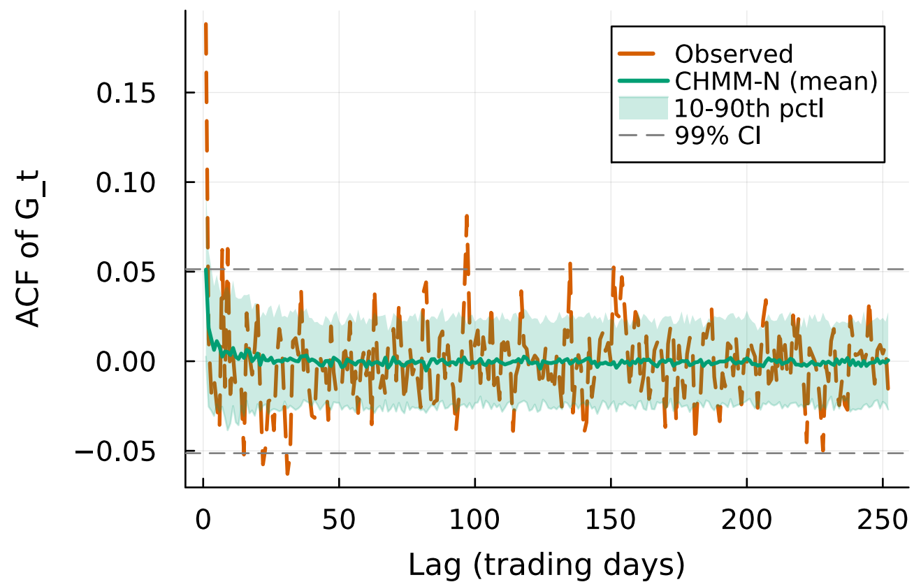
ACF of G_t (raw returns)
