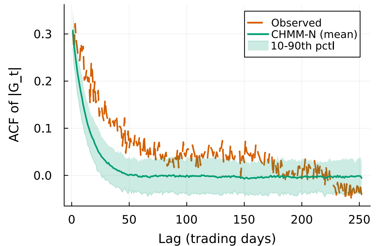
ACF of |G_t|
