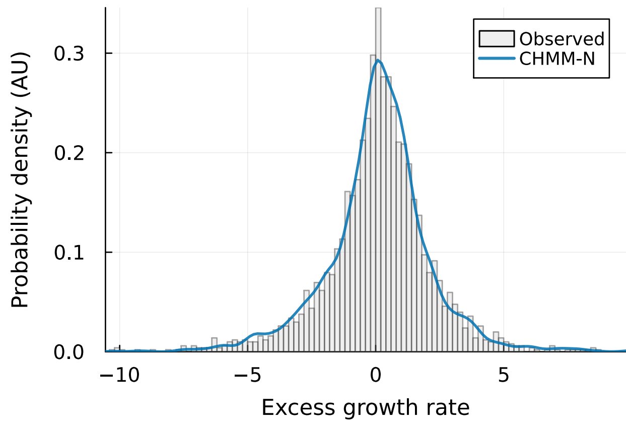
IS density (KS: 94.1%)
