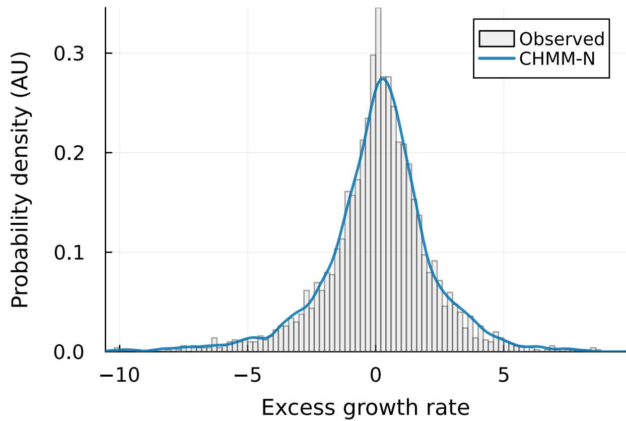
IS density (KS: 95.6%)
