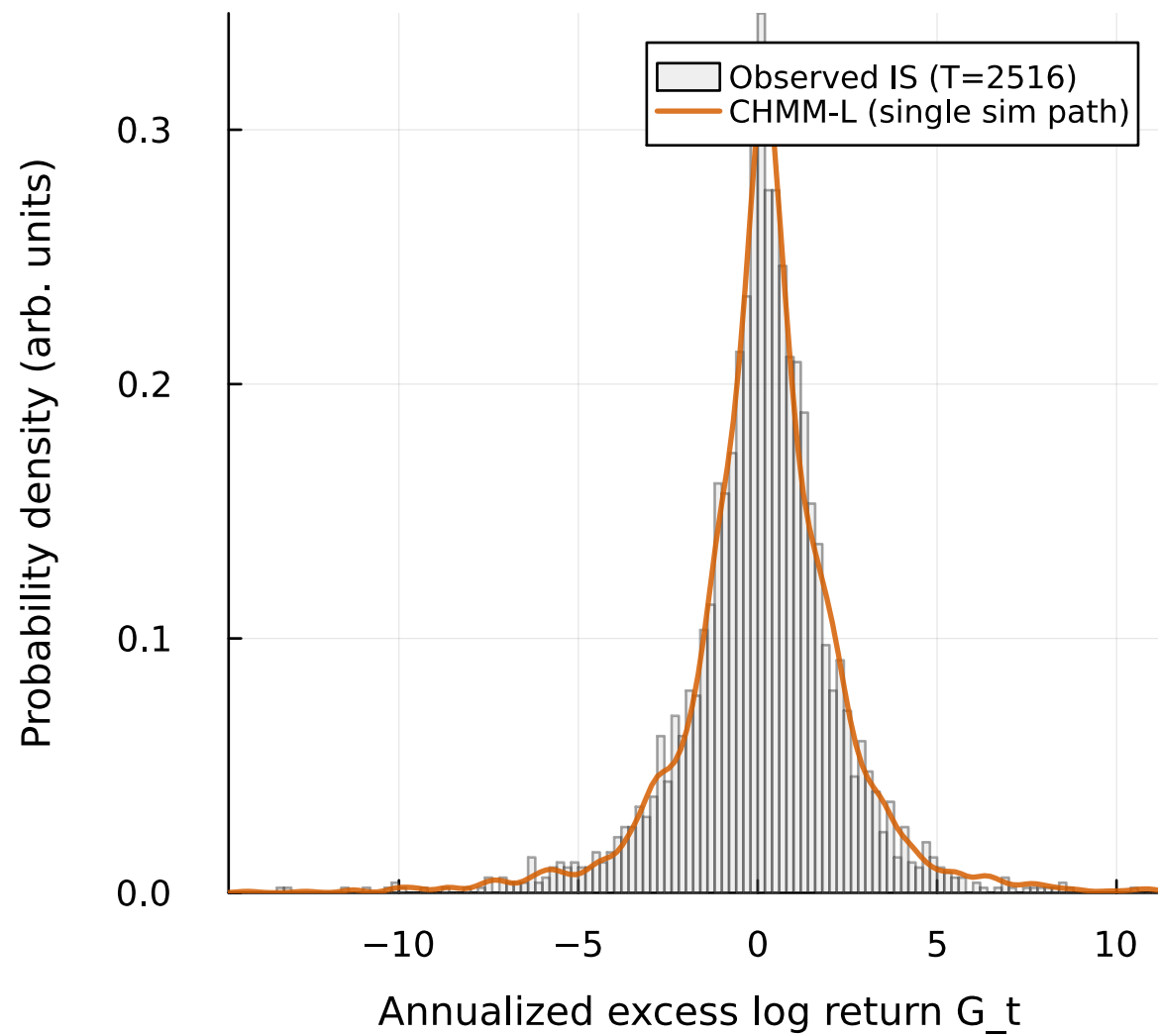
IS return density | KS pass rate = 80.5% of 1000 paths at alpha=0.05
