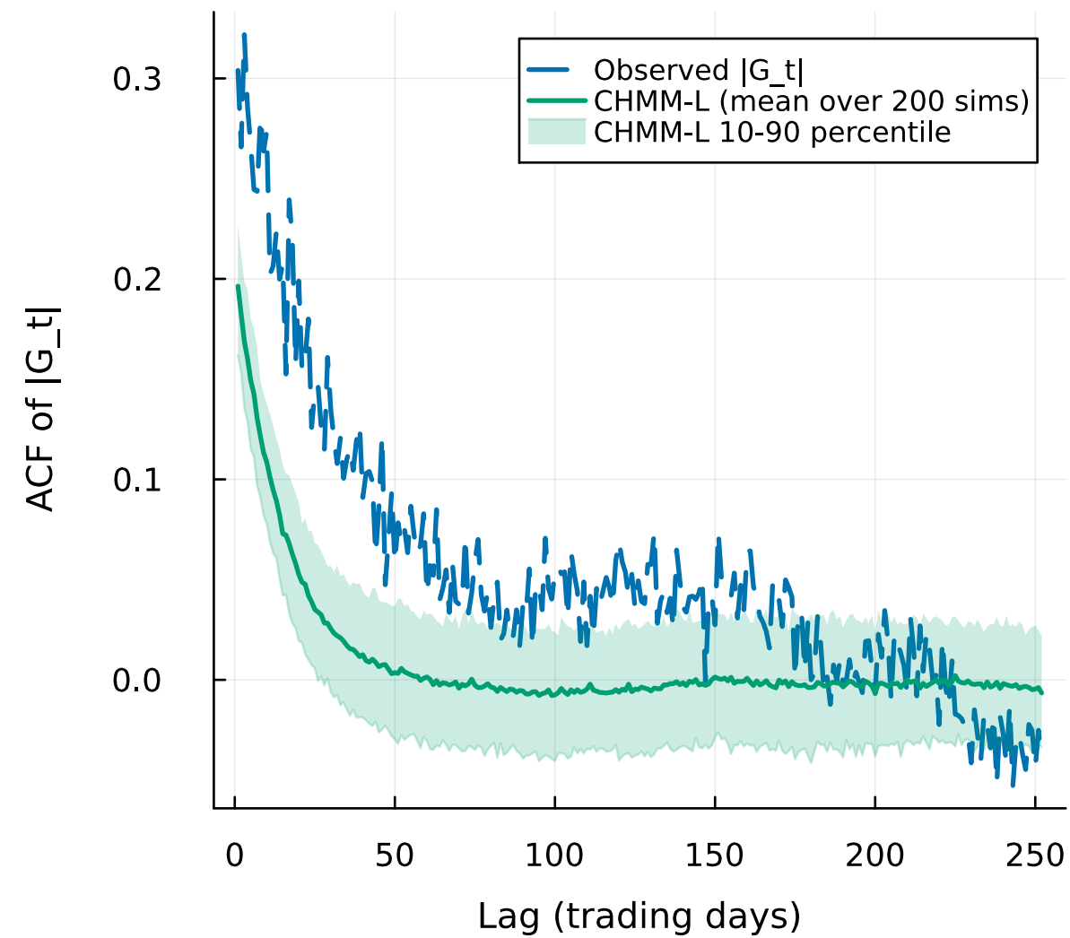
ACF of |G_t| | lag1..252 (trading days)
