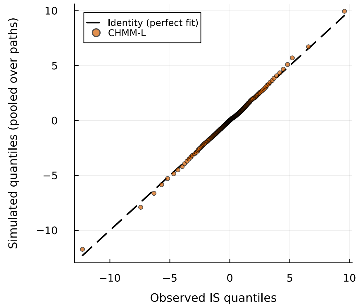
Tail Q-Q plot | quantile grid 0.1% .. 99.9%
