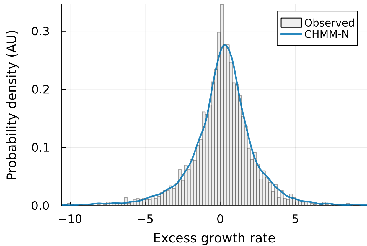
IS density (KS: 90.1%)
