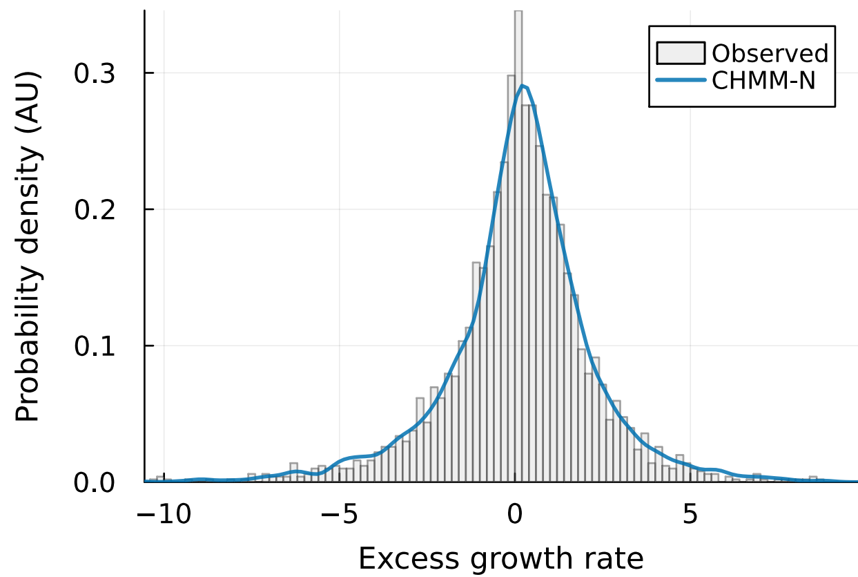
IS density (KS: 90.6%)
