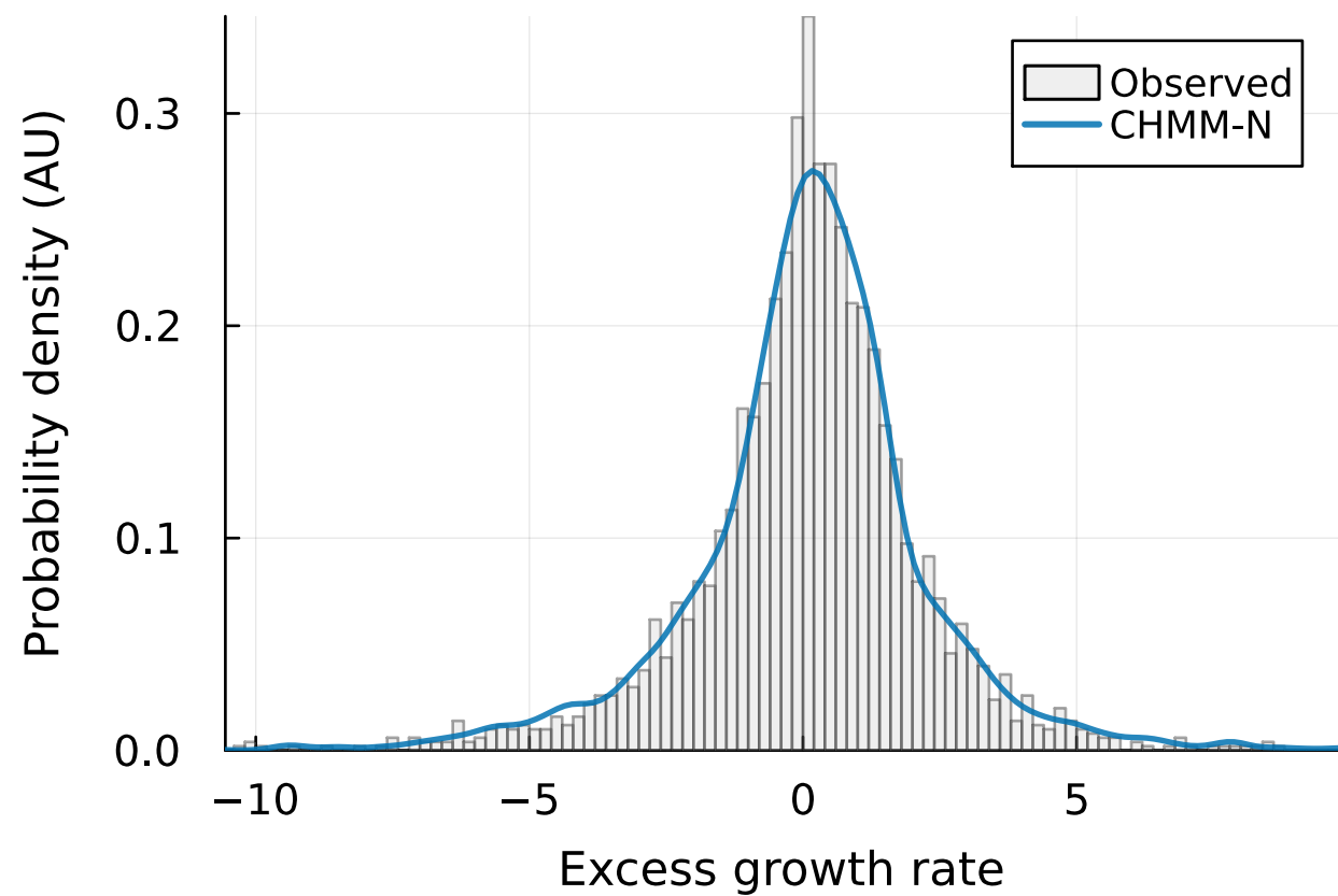
IS density (KS: 93.7%)
