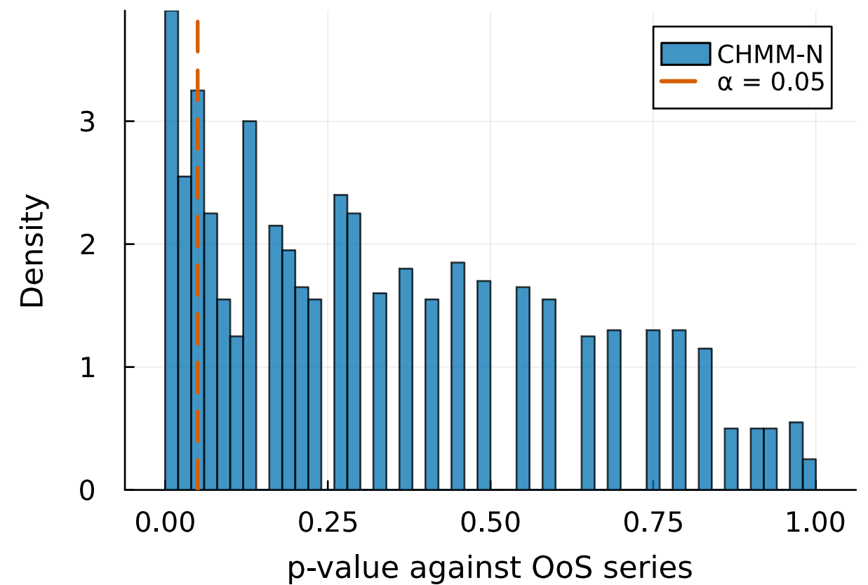
OoS KS p-values (pass: 83.2%)
