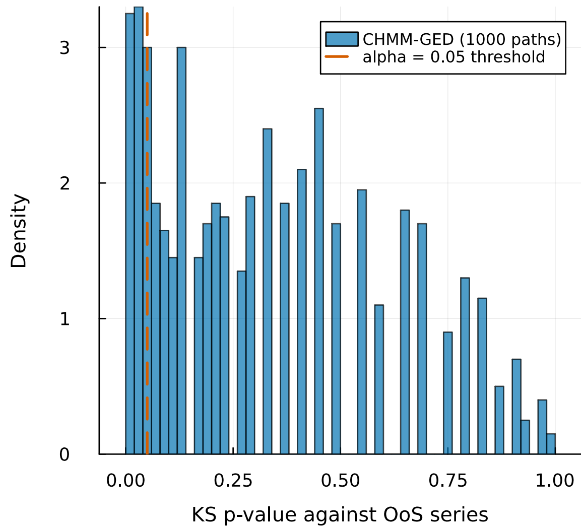
OoS KS p-values | pass rate = 83.8% above alpha=0.05
