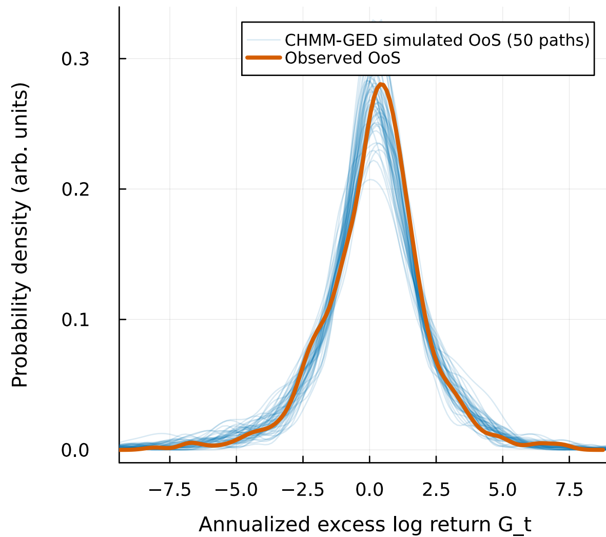
OoS return density fan | 50 sim paths vs. observed OoS (T=572)
