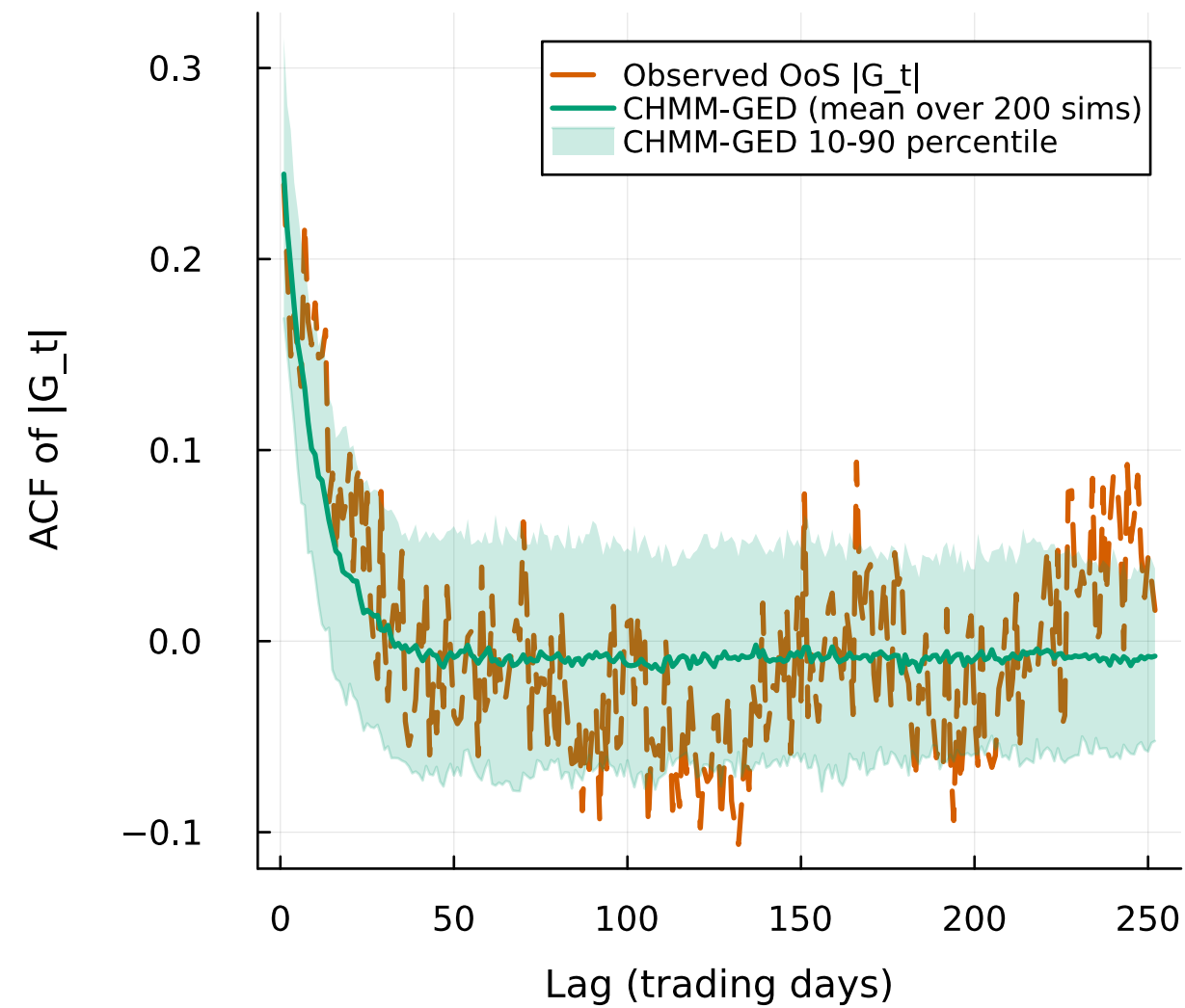
OoS ACF of |G_t| | lag 1..252 (trading days)
