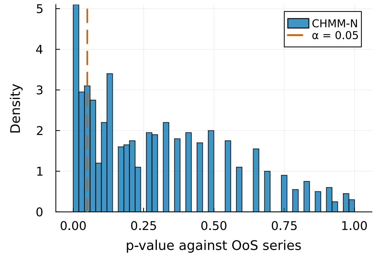
OoS KS p-values (pass: 79.7%)
