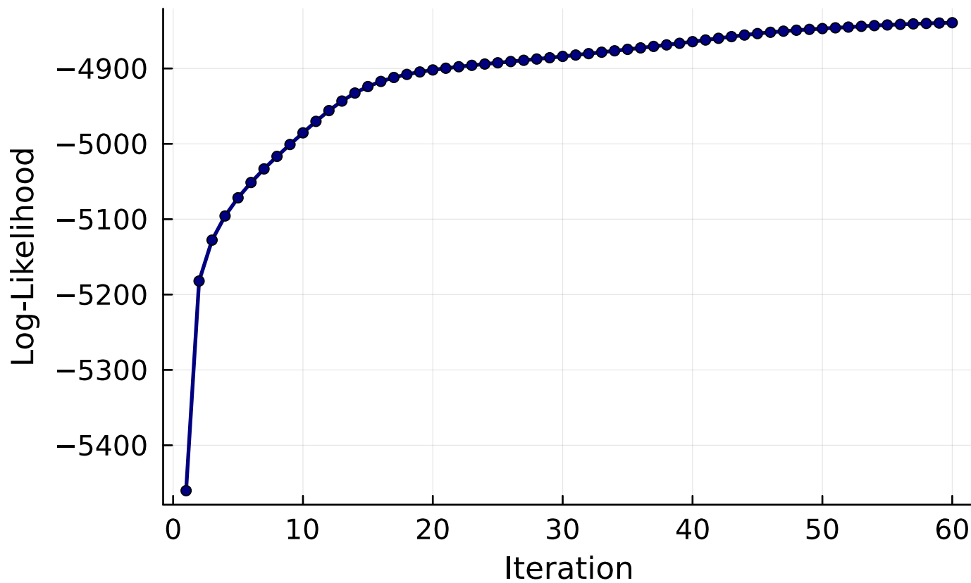
Baum-Welch Convergence (SPY, K=12)
