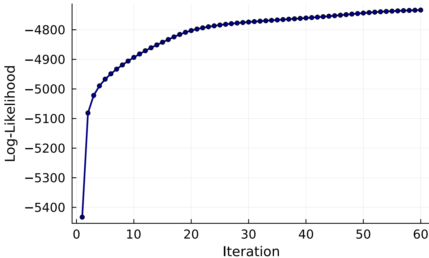
Baum-Welch Convergence (SPY, K=18)
