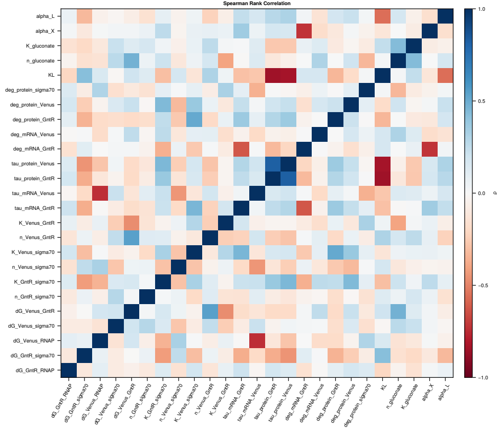
Fig. 7: Spearman rank correlation matrix of the estimated model parameters across the ensemble ( N = 7167 ). Strong positive correlations (blue) and negative correlations (red) reveal parameter dependencies that reflect structural identifiability constraints. Notable correlated clusters include the translation time constants ( \tau_{\text{protein,GntR}} , \tau_{\text{protein,Venus}} ) and the translation saturation constant ( K_L ), which exhibited pairwise correlations |\rho| > 0.82 , reflecting the well-known trade-off between Michaelis constant and time constant in enzyme kinetics. The mRNA degradation modifier for GntR was strongly anti-correlated with \alpha_X ( \rho = -0.72 ), indicating a compensatory relationship between mRNA stability and transcriptional resource depletion rate.
