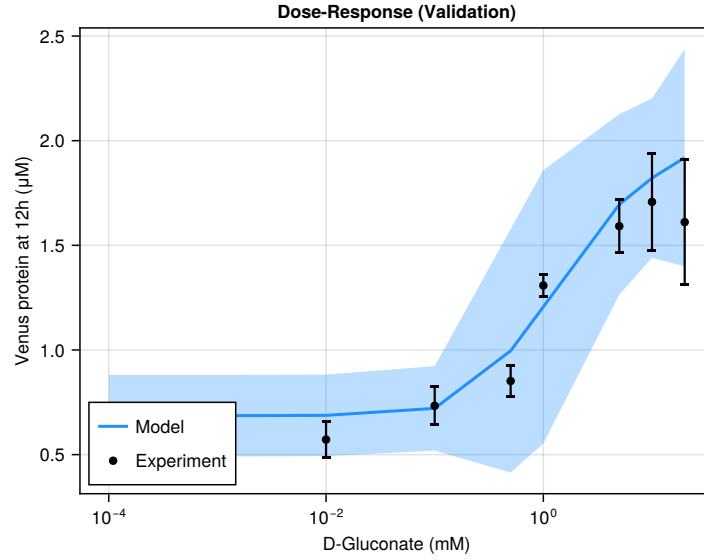
Fig. 5: Model prediction versus experimental measurements for the dose-response study. Linear DNA used were: mP70-Venus (7 nM), P70-GntR (10 nM). D-gluconate concentration was varied from 0.0001 to 20 mM. Black circles represent Venus protein measurements at the endpoint of the experiment (12 h). Error bars represent standard errors across at least three replicates. The black line represents the ensemble mean of the model prediction, and the shaded region represents the 95% confidence estimate across the parameter ensemble ( N = 7167 ). All model parameters were fixed at the values estimated from the 10 mM and 0 mM D-gluconate training conditions; only D-gluconate concentration was varied.
