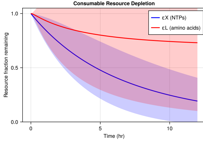
Fig. 4: Predicted trajectories of consumable resource availability over the 12-hour cell-free reaction. The transcriptional resource variable \epsilon_X (representing the fractional availability of nucleotides and energy cofactors for transcription) and the translational resource variable \epsilon_L (representing the fractional availability of amino acids and energy cofactors for translation) were computed from the mechanistic resource depletion model (Eqns. 14–15). By 12 hours, \epsilon_X declined to 0.19 (81% depletion) while \epsilon_L declined to 0.74 (26% depletion), indicating that transcriptional resources were the primary bottleneck. Lines represent the ensemble mean; shaded regions represent the 95% confidence interval across the parameter ensemble ( N = 7167 ).
