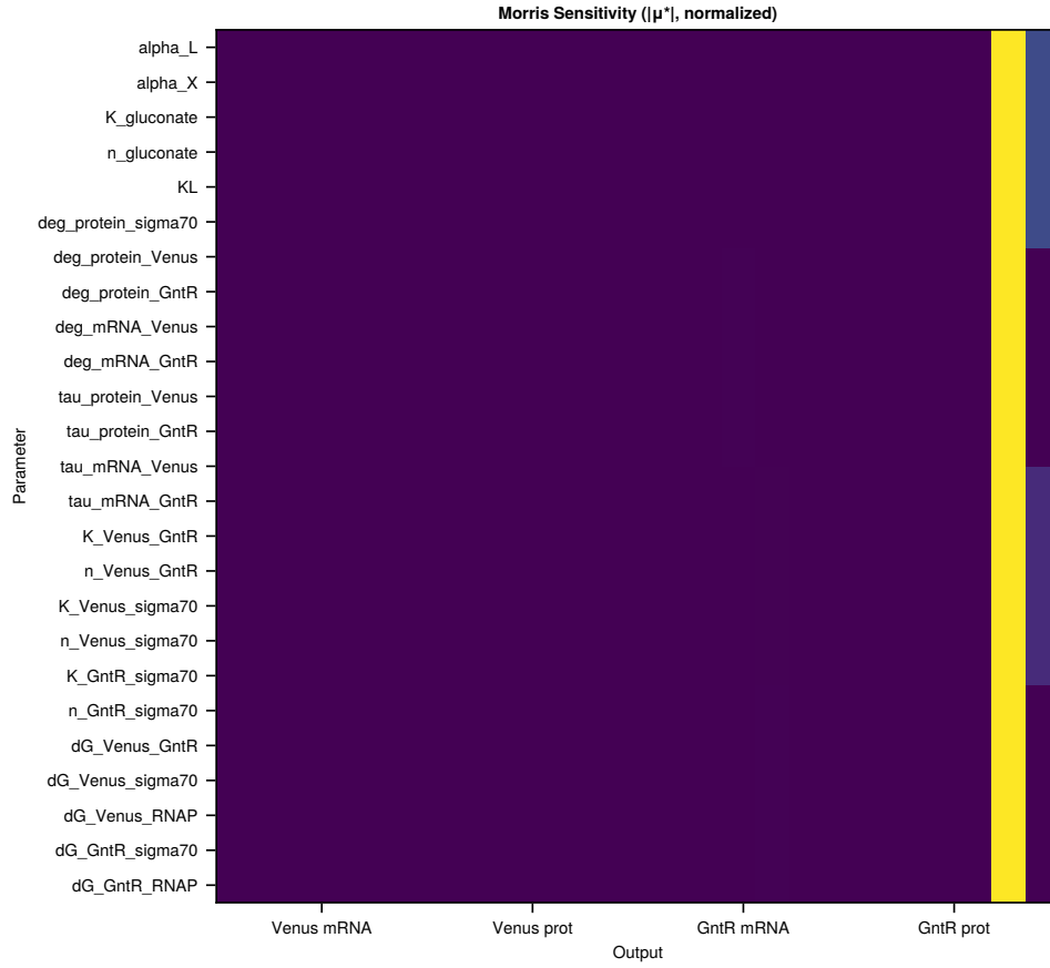
Fig. 6: Global sensitivity analysis of the model parameters using the Morris method. The heatmap represents the normalized absolute mean elementary effect ( |\mu^*| ) of each parameter on four model outputs: Venus mRNA at 6 hours, Venus protein at 12 hours, GntR mRNA at 6 hours, and GntR protein at 12 hours. Values were normalized per output to the range [0, 1] for visualization; darker colors indicate greater sensitivity. The resource consumption parameters \alpha_X and \alpha_L were the dominant parameters for all model outputs. Morris sensitivity coefficients were computed over 200 trajectories using parameter ranges derived from the ensemble distribution.
