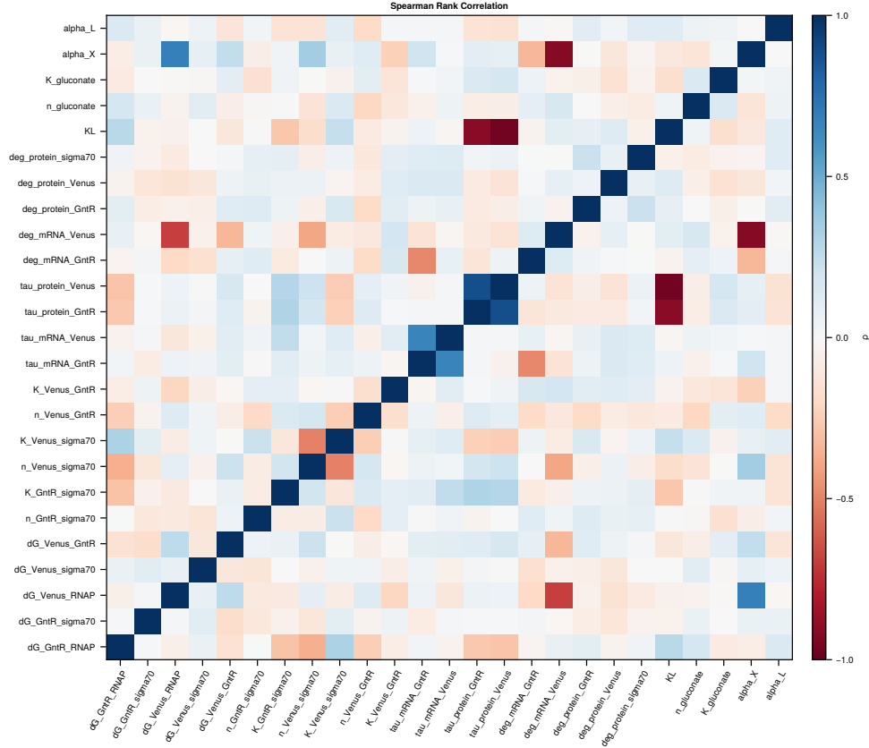
Fig. 7: Spearman rank correlation matrix of the estimated model parameters across the ensemble ( N = 78 ). Strong positive correlations (blue) and negative correlations (red) reveal parameter dependencies that reflect structural identifiability constraints. Notable correlated clusters include the translation time constants ( \tau_{\text{protein,GntR}} , \tau_{\text{protein,Venus}} ) and the translation saturation constant ( K_L ), which exhibited pairwise correlations |\rho| > 0.82 , reflecting the well-known trade-off between Michaelis constant and time constant in enzyme kinetics. The mRNA degradation modifier for GntR was strongly anti-correlated with \alpha_X ( \rho = -0.72 ), indicating a compensatory relationship between mRNA stability and transcriptional resource depletion rate.
