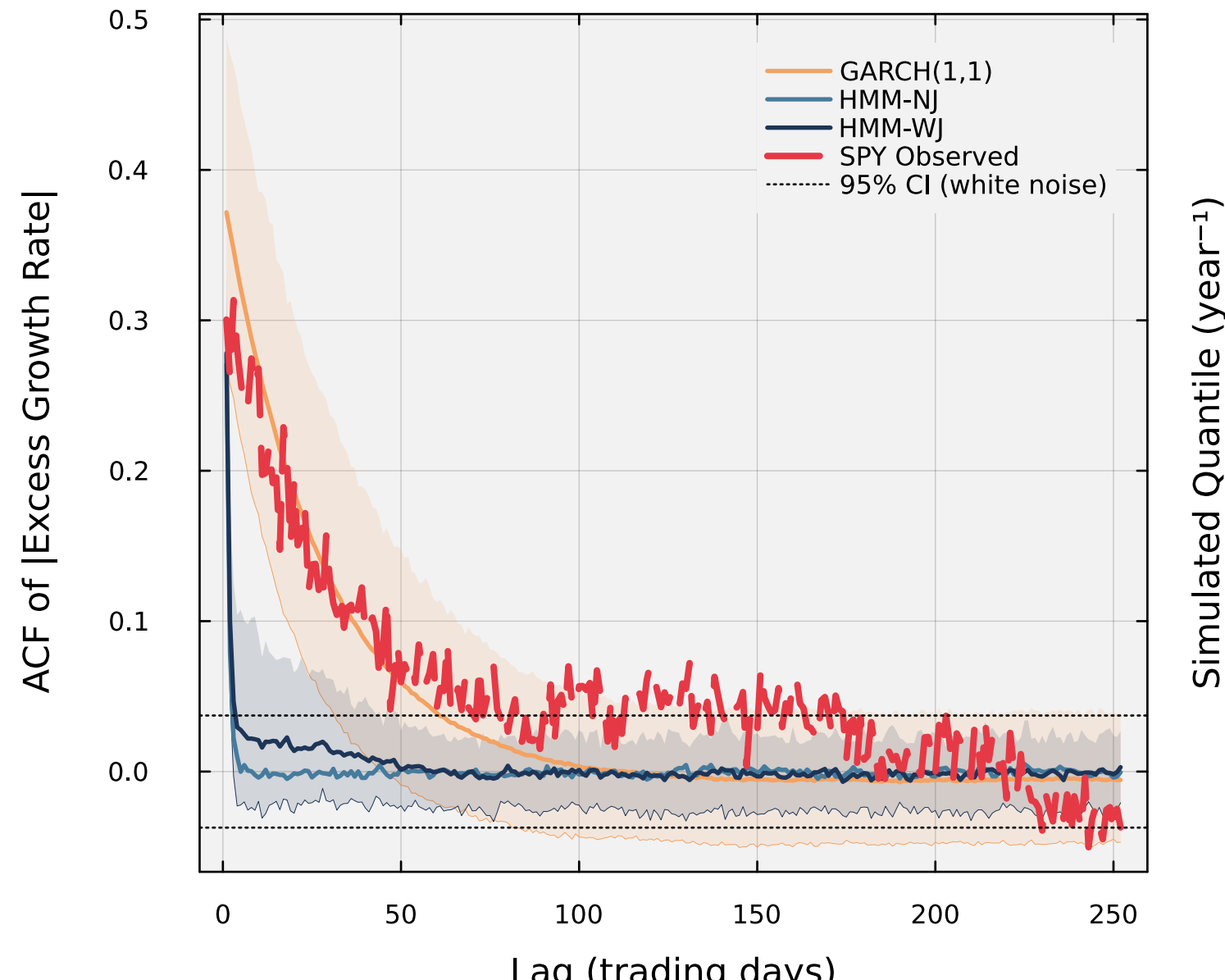
(b) Volatility Clustering (ARCH Effect)
