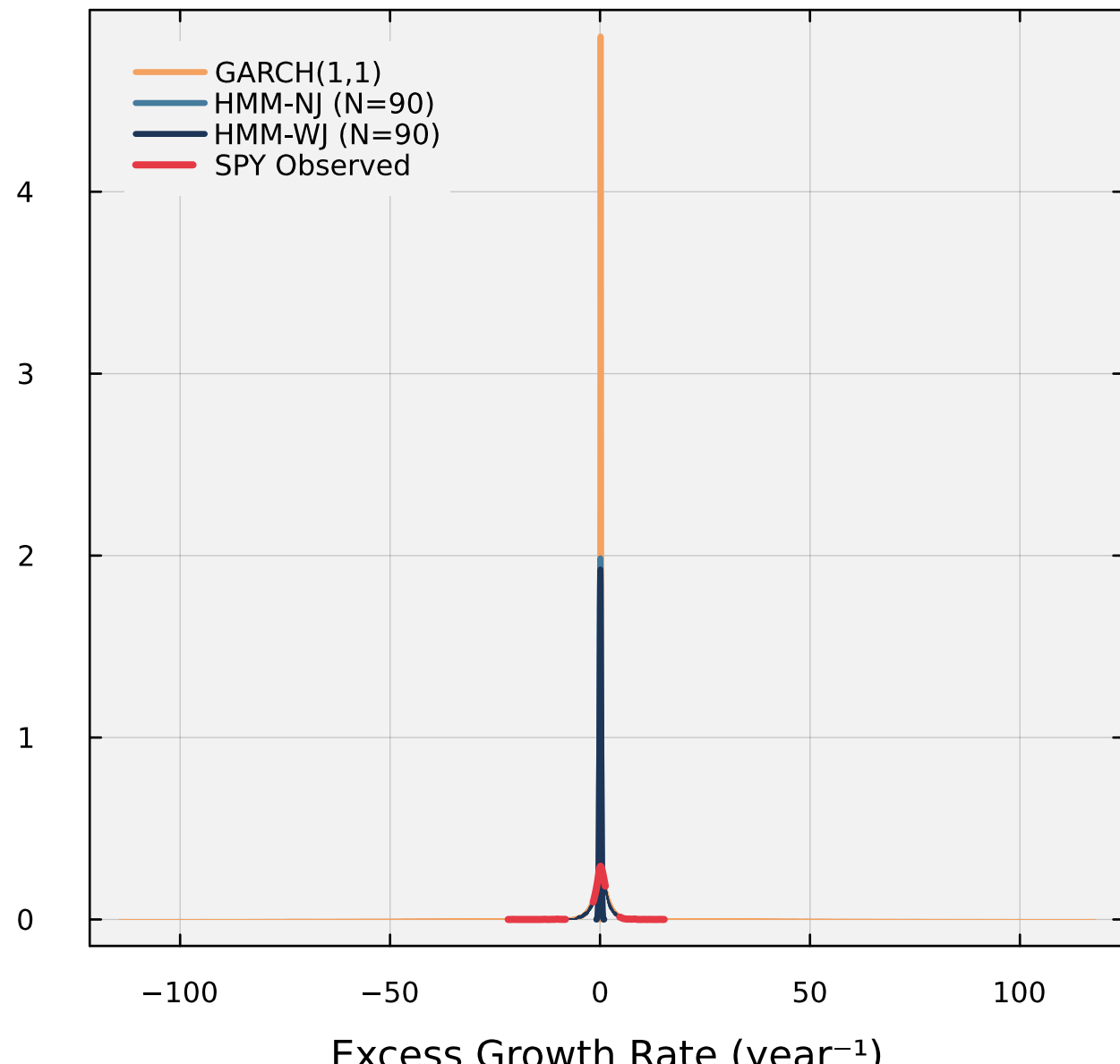
(a) Marginal Distributions
