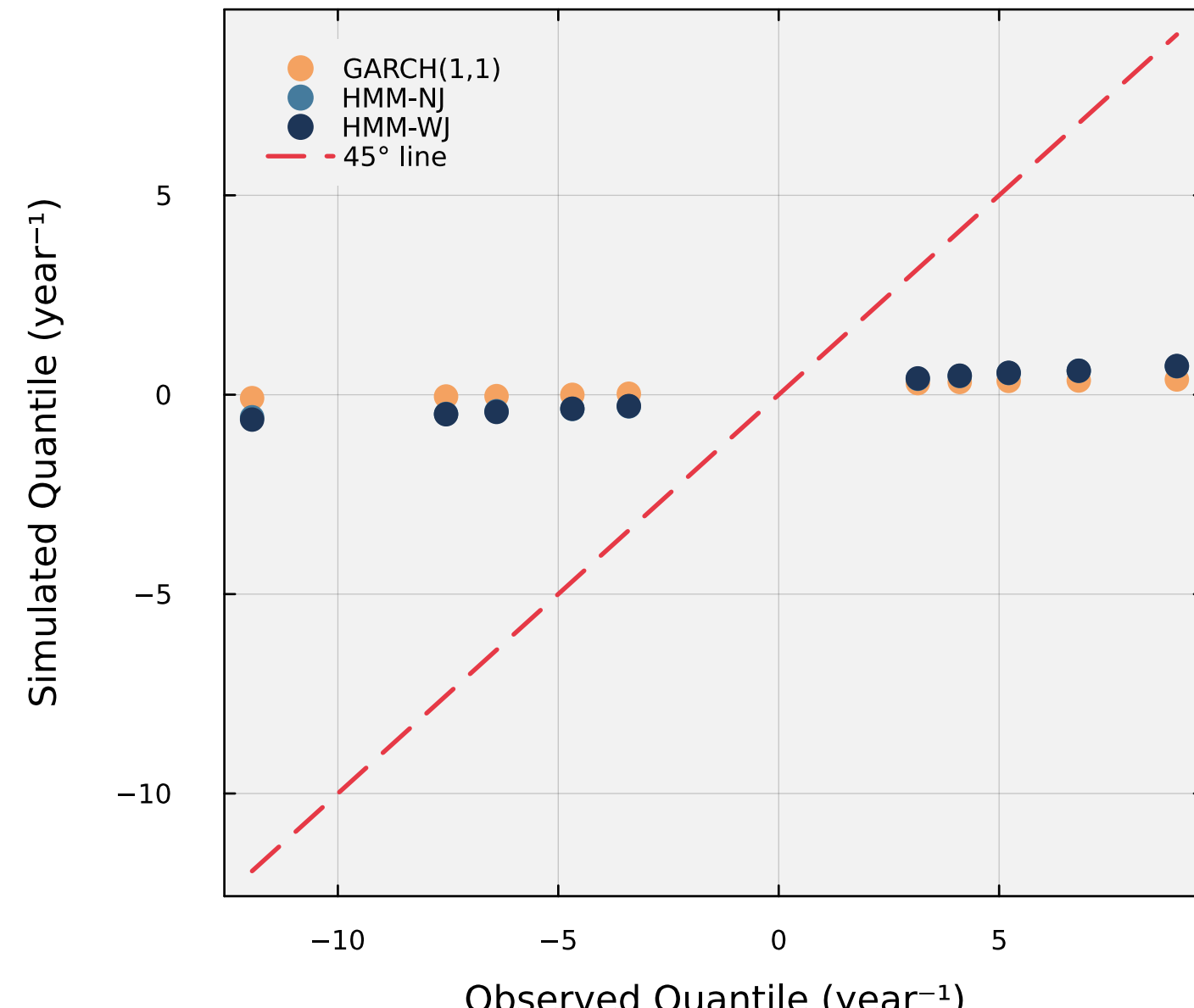
(c) Tail Q-Q Plot
