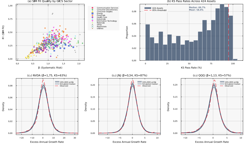
Fig. 5. Multi-asset extension via the Single-Index Model (SIM) across 424 S&P 500 constituents. Panel (a) summarizes the SIM regression fit quality by GICS sector. Panel (b) shows that KS distributional consistency is maintained across the full asset universe when paths are generated via the factor structure \hat{G}_{i,t} = \hat{\alpha}_i + \hat{\beta}_i G_{SPY,t} + \hat{\eta}_{i,t} . Panel (c) illustrates representative marginal density comparisons for three assets spanning a wide range of systematic risk exposure.
