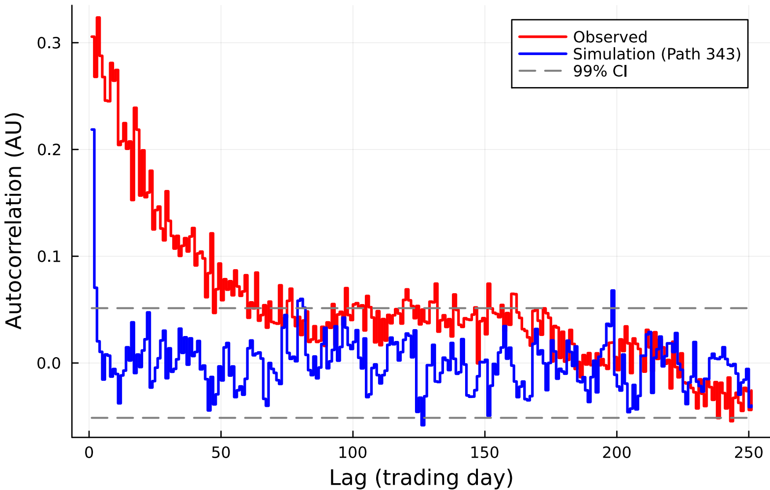
ACF of SPY |Growth Rate| (No-Jumps, Path 343)
