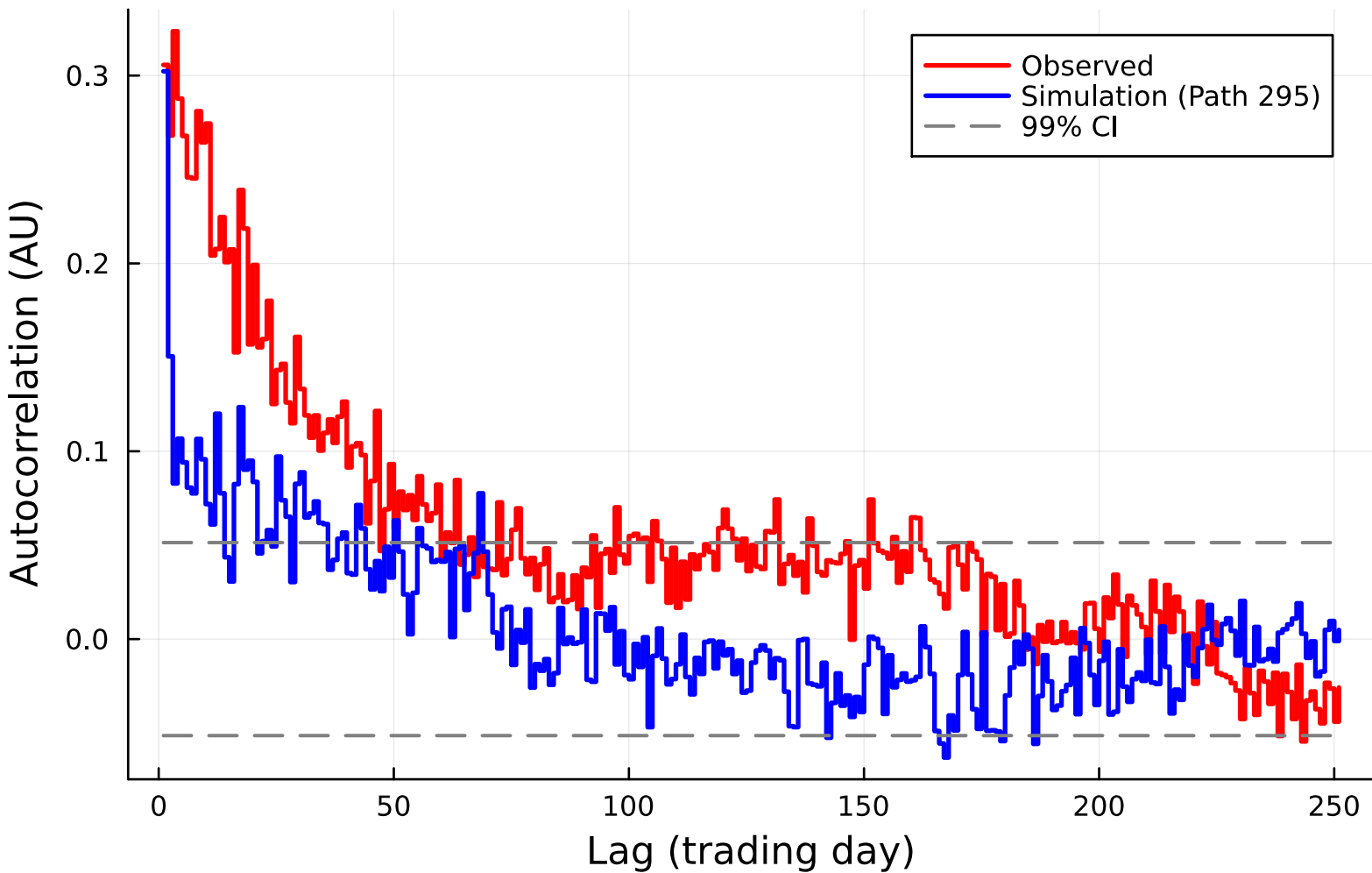
ACF of SPY |Growth Rate| (Jump, Path 295)
