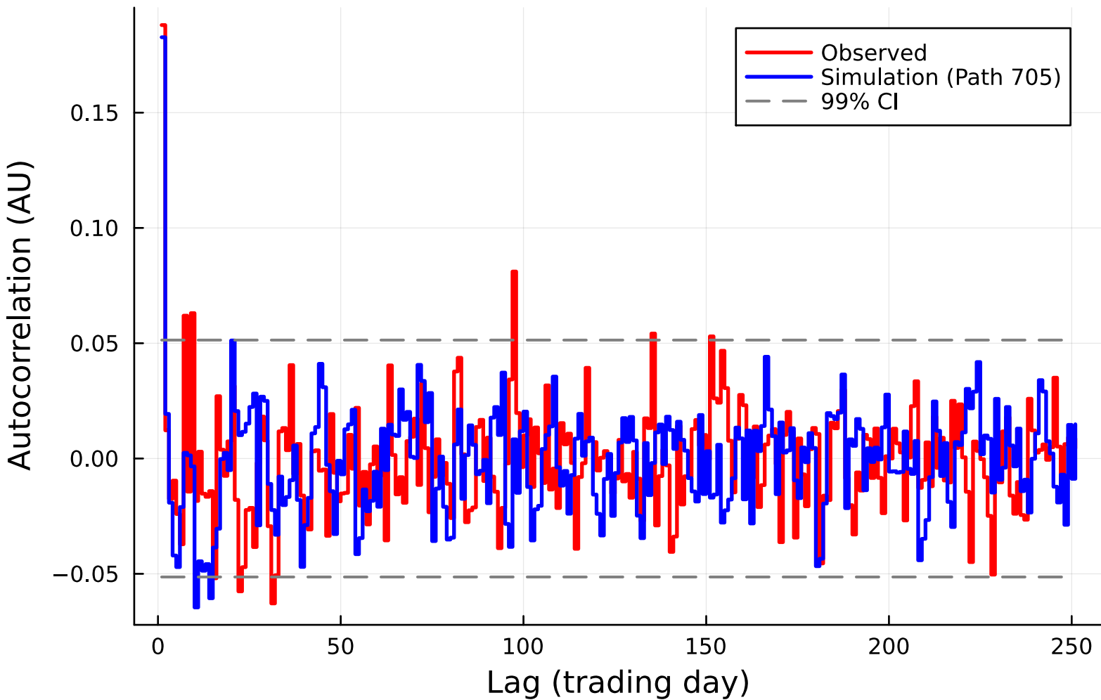
ACF of SPY Growth Rate (Non-Jump, Path 705)
