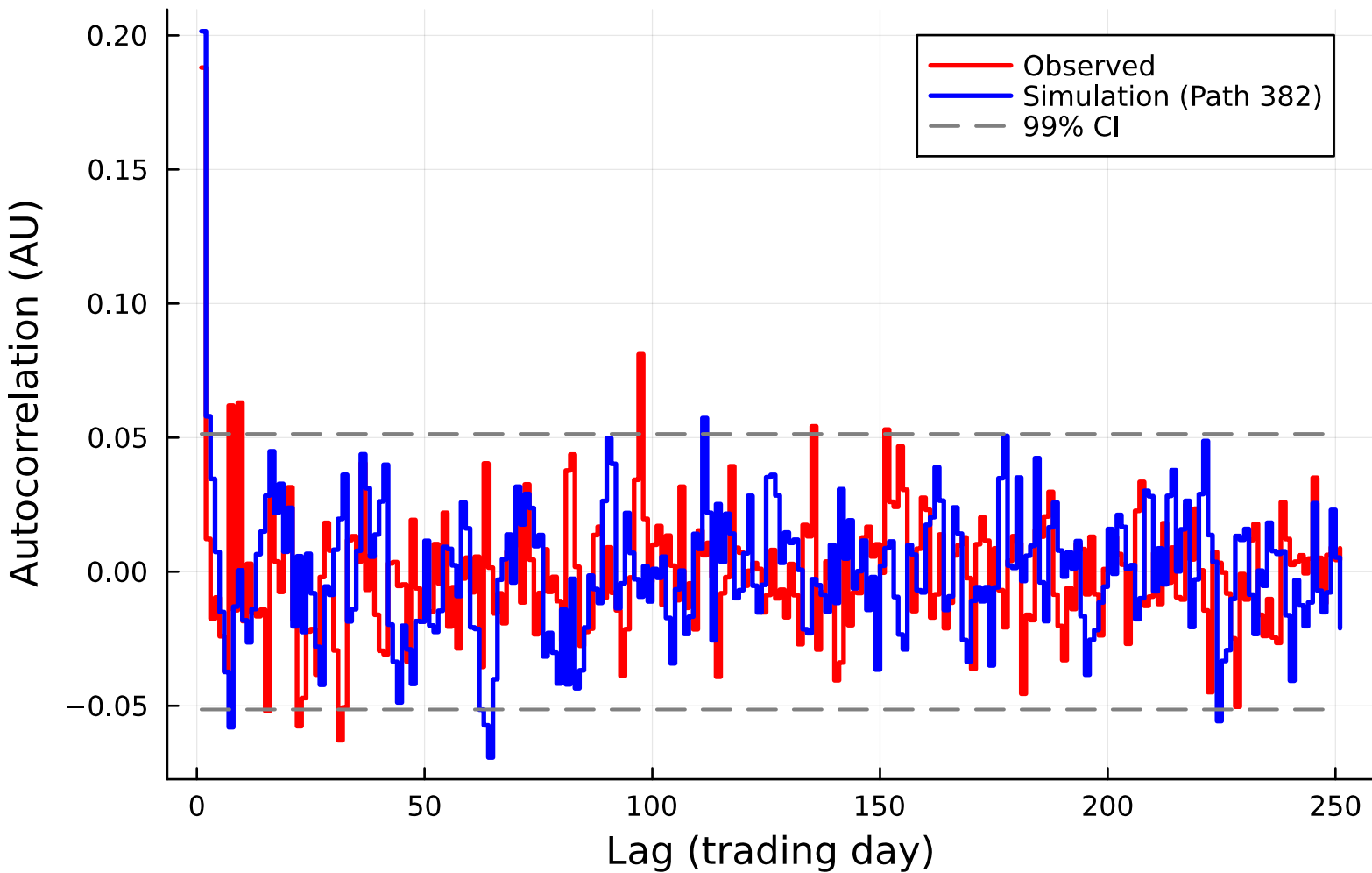
ACF of SPY Growth Rate (Non-Jump, Path 382)
