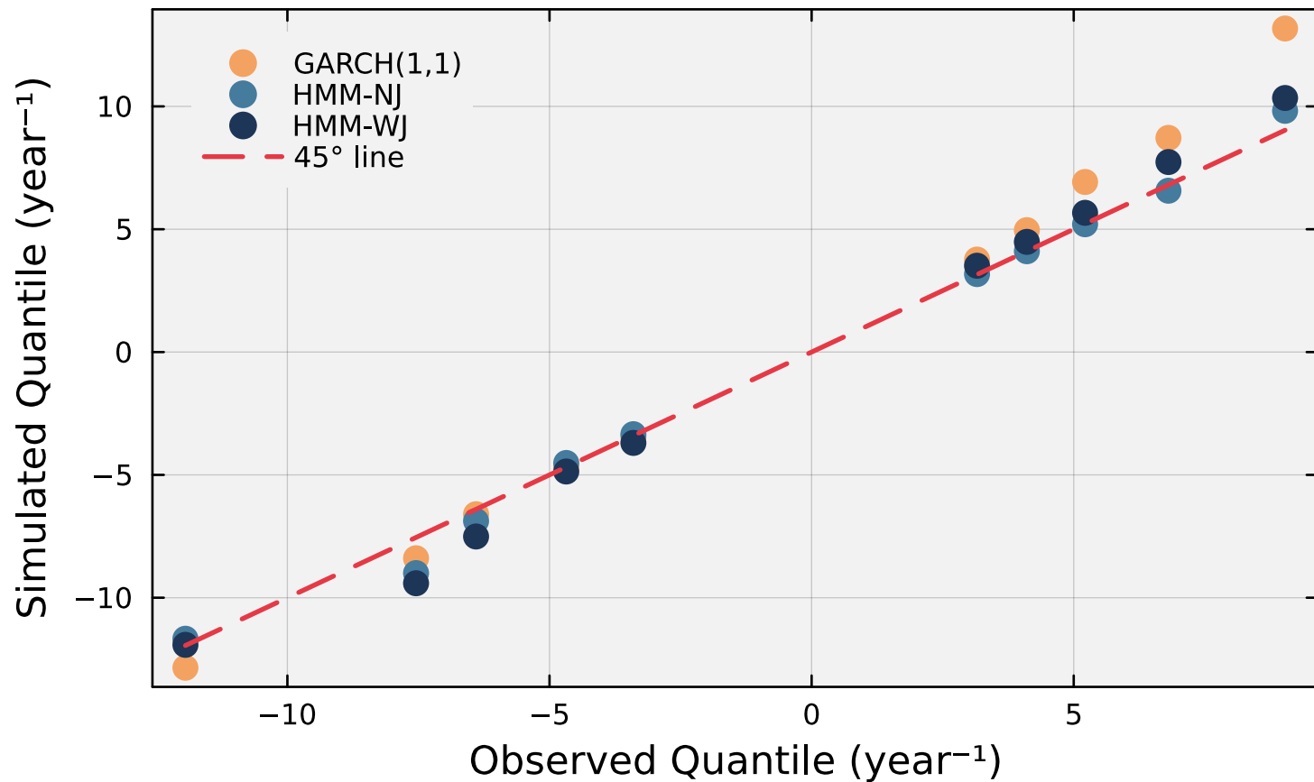
(c) Tail Q-Q Plot
