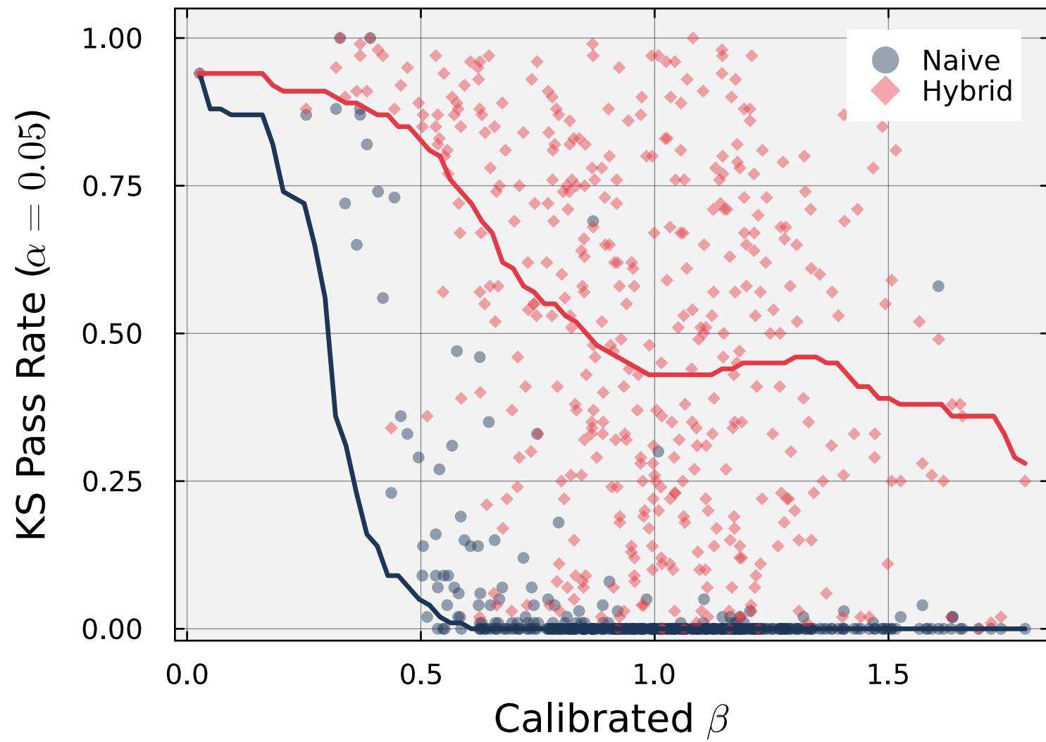
(a) KS Pass Rate per Ticker
