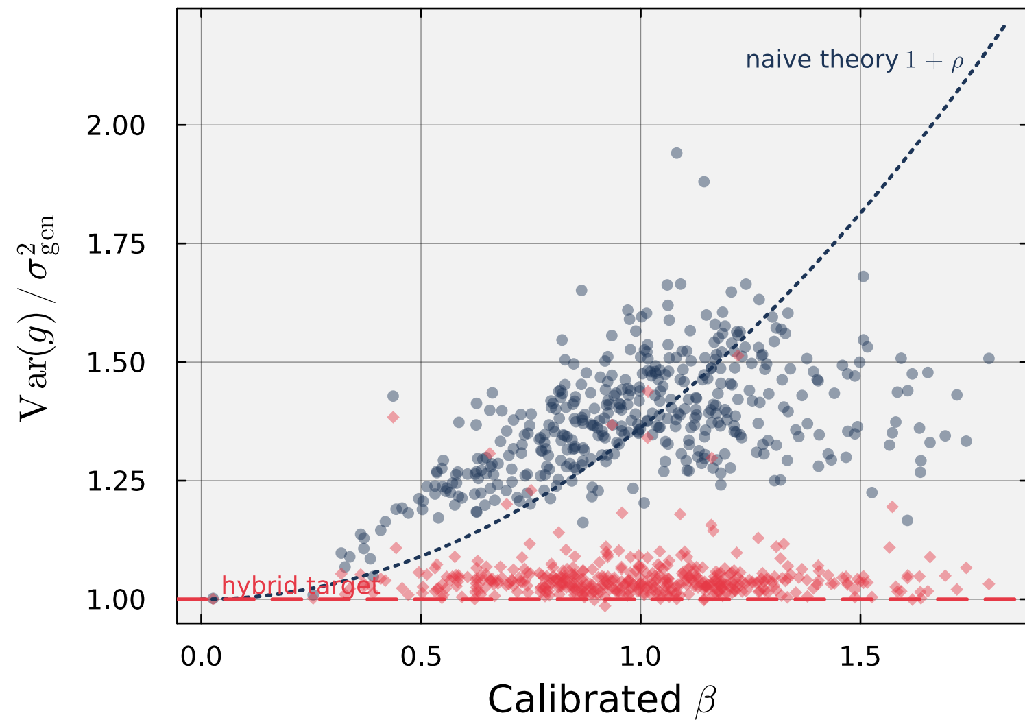
(b) Variance Preservation
