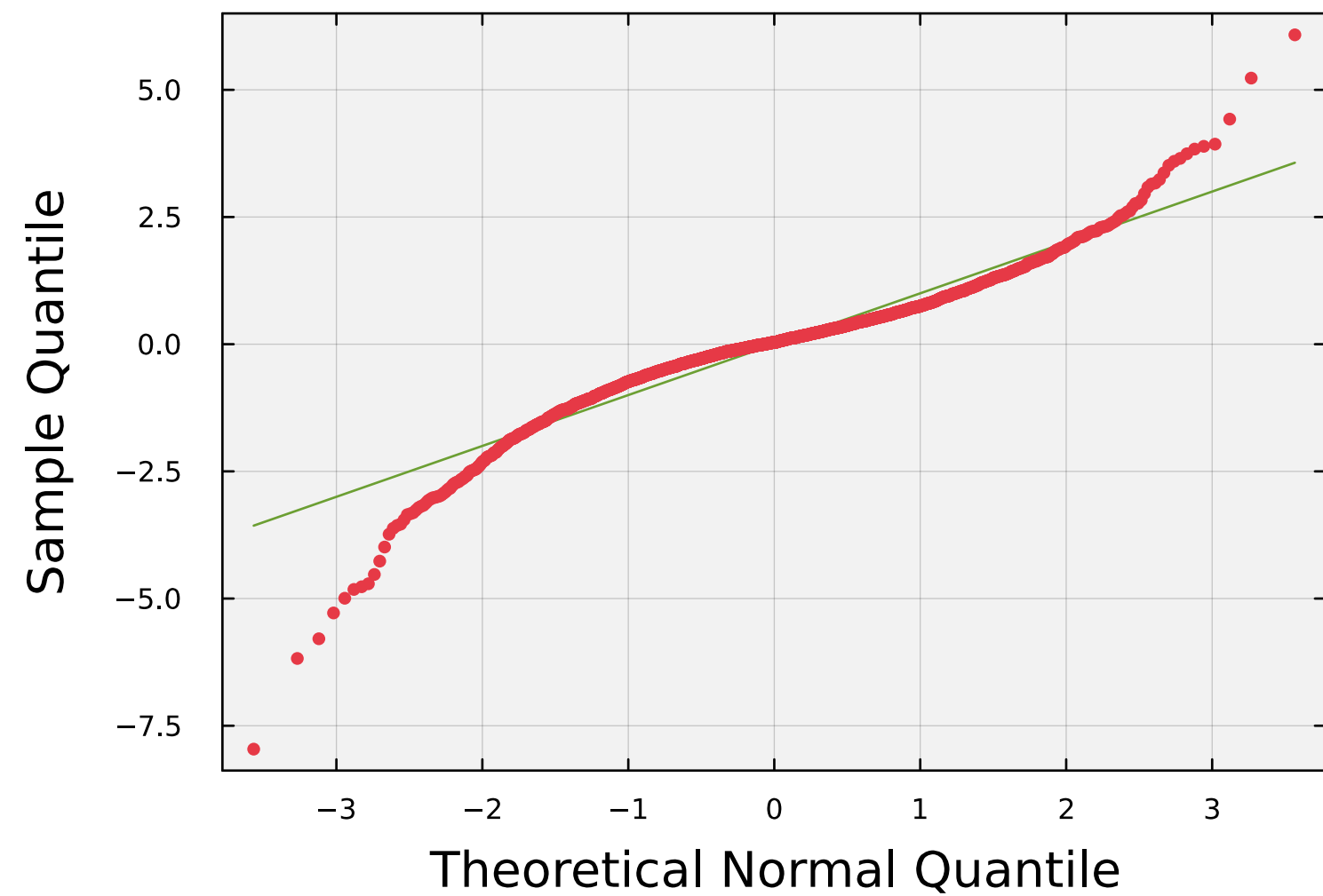
(b) Normal Q-Q Plot
