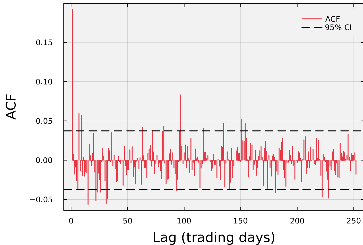
(c) ACF of Raw Excess Growth Rates
