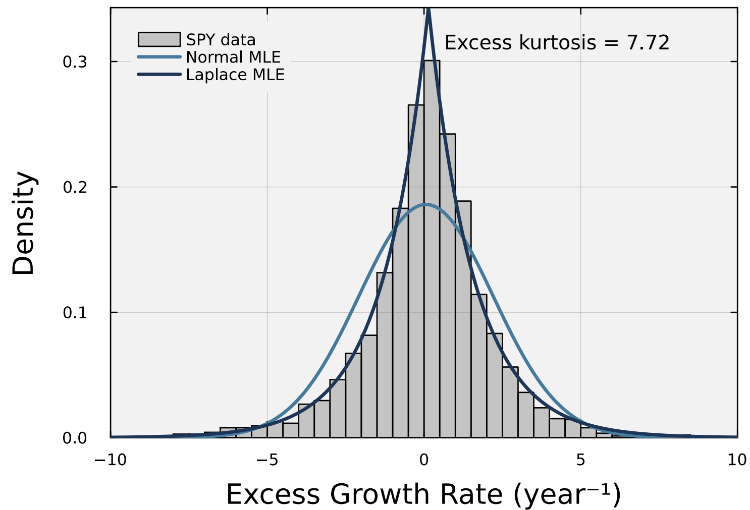
(a) Marginal Distribution
