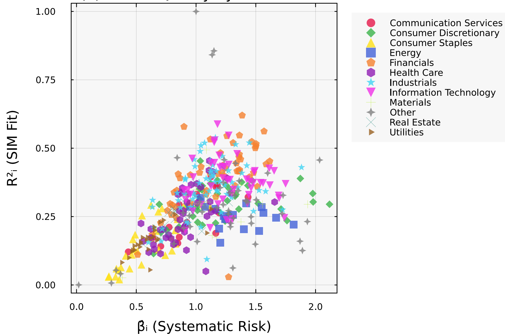
(a) SIM Fit Quality by GICS Sector
