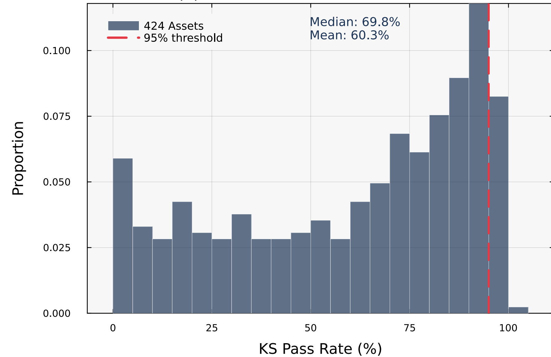
(b) KS Pass Rates Across 424 Assets
