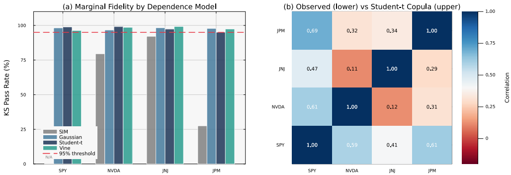
Fig. 6. Dependence model comparison for the four-asset portfolio (SPY, NVDA, JNJ, JPM). Panel (a): KS pass rates by ticker and dependence model. All three copula specifications preserve per-asset marginal fidelity above 95%, while the SIM degrades to 27.5% for JPM due to low factor loading ( R^2 = 0.48 ). The dashed line marks the 95% threshold. Panel (b): observed pairwise correlations (lower triangle) vs. Student-t copula simulated correlations (upper triangle). The Student-t copula reproduces the cross-asset dependence structure with a pairwise MAE of 0.039; the largest discrepancy is SPY-JNJ (observed 0.47, simulated 0.41).
