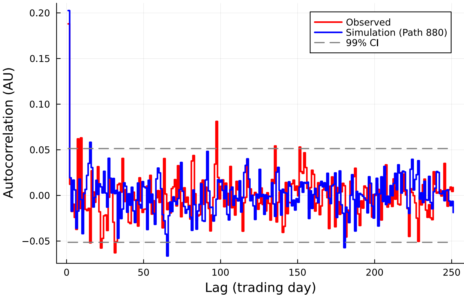
ACF of SPY Growth Rate (Non-Jump, Path 880)
