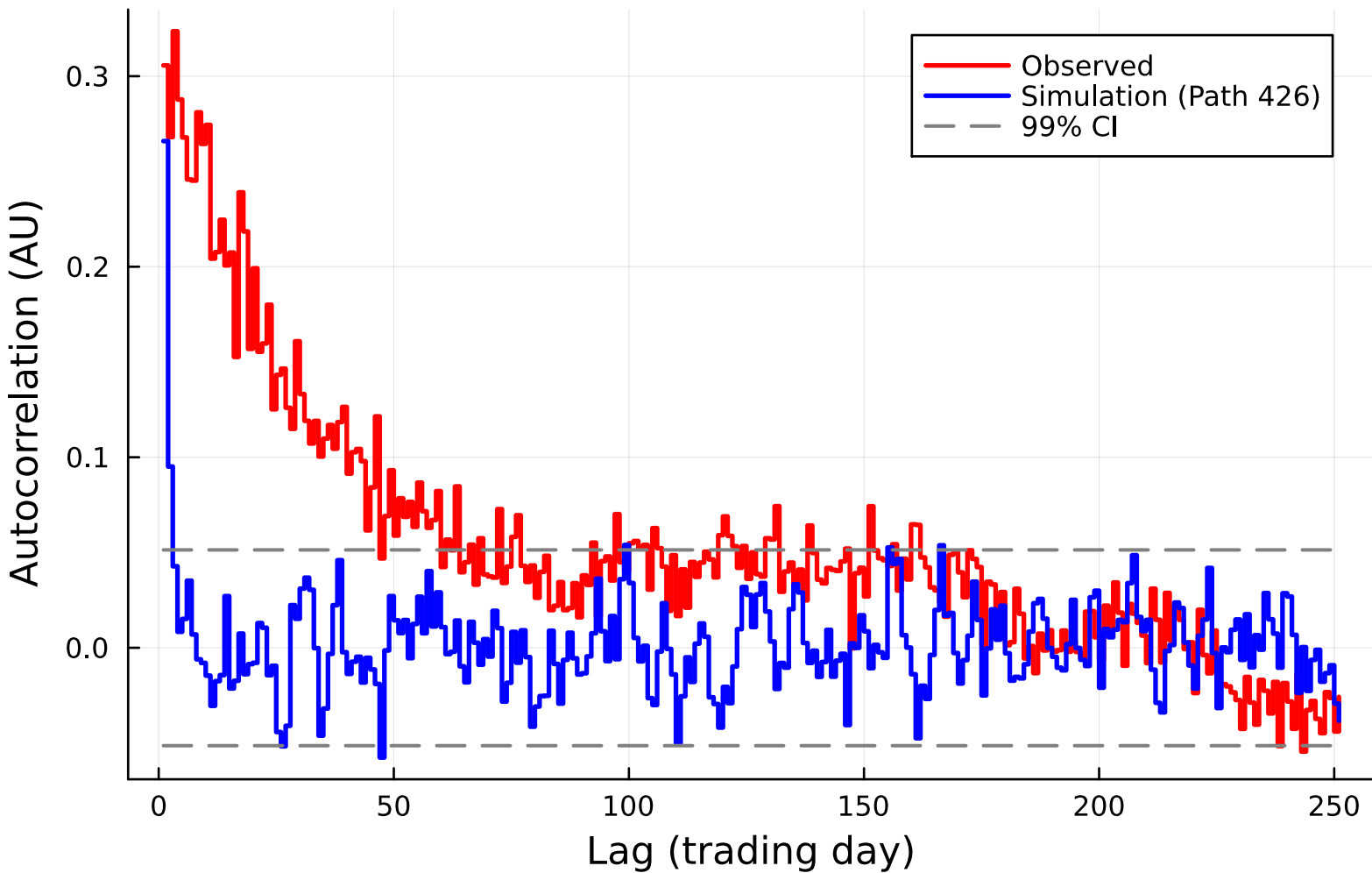
ACF of SPY |Growth Rate| (No-Jumps, Path 426)
