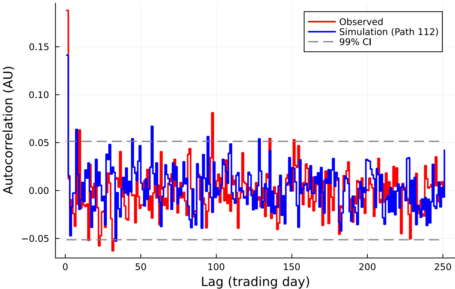
ACF of SPY Growth Rate (Jump, Path 112)
