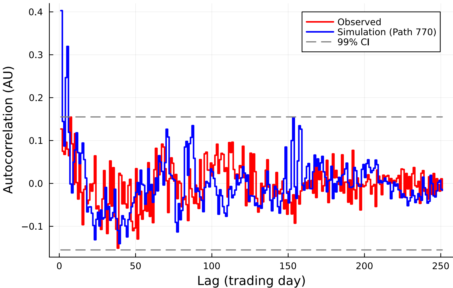
ACF of SPY [Growth Rate] (Jump, Path 770)
