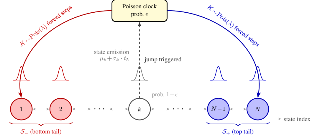
Figure 2: Architecture of the hybrid hidden Markov model with a jump-duration mechanism (HMM-WJ). When no jump episode is active, the chain transitions according to the empirical transition matrix \mathbf{T} with probability 1 - \epsilon (thin bidirectional arrows) or enters a Poisson jump episode with probability \epsilon (dashed upward arrow to the Poisson clock). During an episode, each of the K \sim \text{Pois}(\lambda) forced steps independently draws the bottom tail set \mathcal{S}_- (red, lowest-valued states) with probability p_{\text{neg}} or the top tail set \mathcal{S}_+ (blue, highest-valued states) otherwise, before normal Markovian evolution resumes. Small bell curves above each state depict the state-conditional location-scale Student- t ( \nu = 5 ) emission distribution. Tail sets are defined as the N_{\text{tail}} lowest- and highest-quantile states under the Laplace quantile partition.
