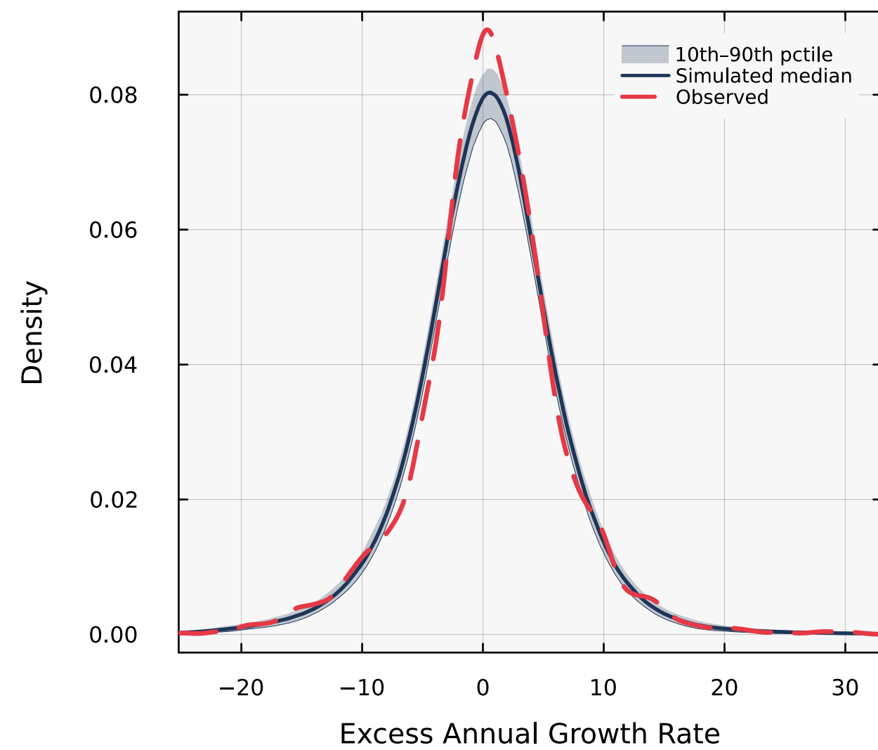
(c 1 ) NVDA ( \beta=1.75 , KS=63%)
