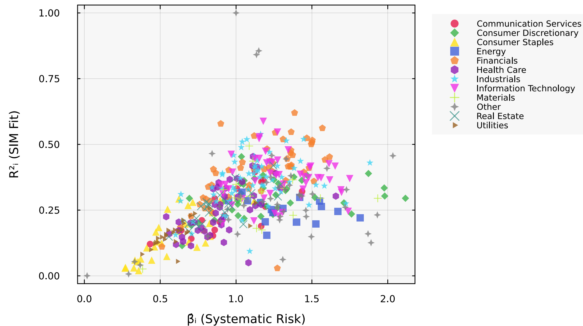
(a) SIM Fit Quality by GICS Sector
