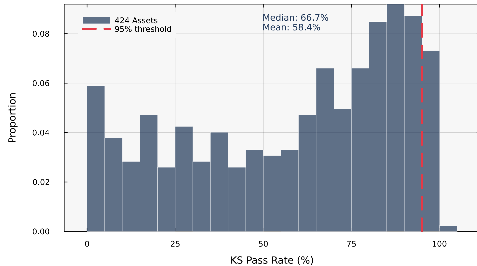
(b) KS Pass Rates Across 424 Assets
