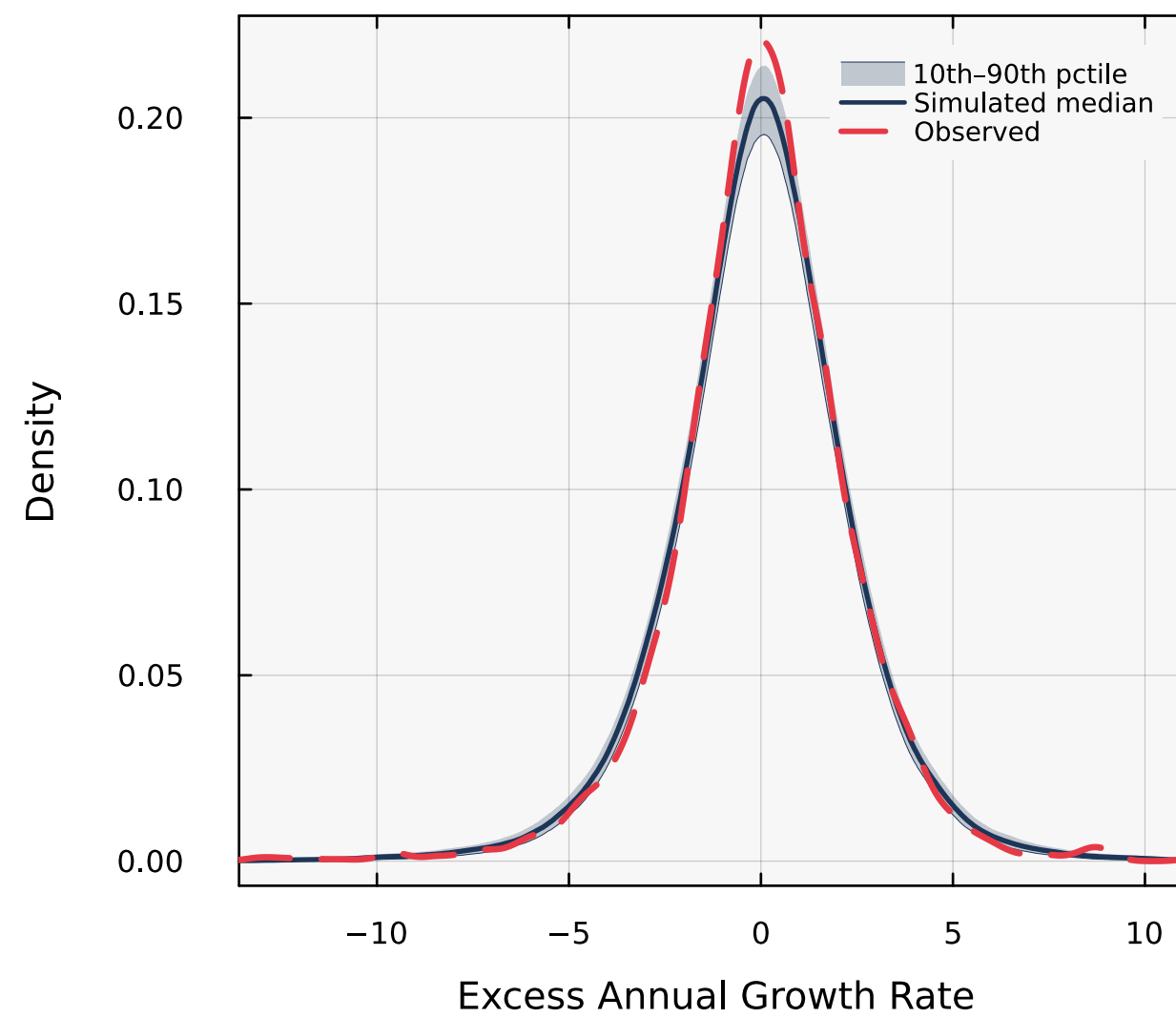
(c 2 ) JNJ ( \beta=0.54 , KS=87%)
