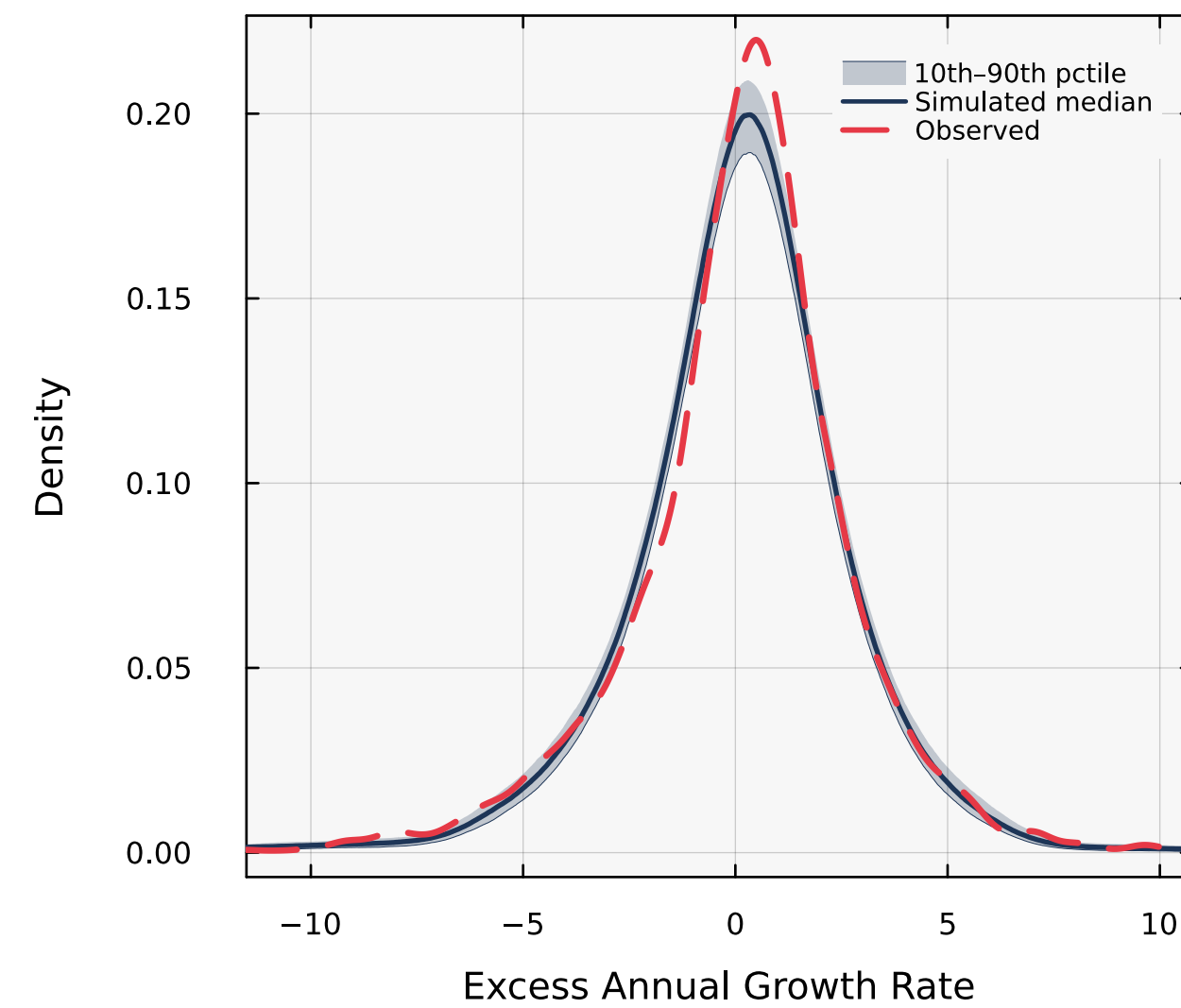
(c 3 ) QQQ ( \beta=1.13 , KS=57%)
