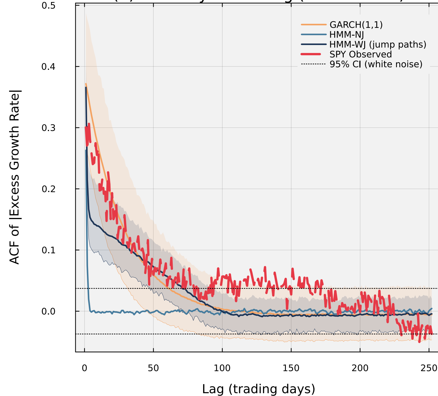
(b) Volatility Clustering (ARCH Effect)
