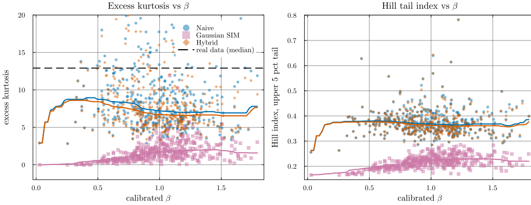
Figure S1: Heavy-tail preservation: excess kurtosis and Hill tail index vs calibrated \beta . Each point is a per-ticker median over 100 replications. Left: excess kurtosis, y -axis clipped to [-2, 20] for readability. The dashed line marks the median real-data excess kurtosis across the universe ( \kappa_{\text{real}} \approx 13 ); the hybrid and naive composition methods (orange and blue) track each other, while the Gaussian single-index model (SIM) stays near \kappa \approx 1 . Right: Hill tail-index estimator on the upper 5% of |g| . The hybrid and naive medians remain near 0.37 throughout the \beta range; Gaussian SIM sits near 0.22. The shortfall from \kappa_{\text{real}} is present with and without variance correction; this similarity does not isolate the effect of rescaling. Both composed distributions depend on the market and generator variance shares (Eq. (S53)).
