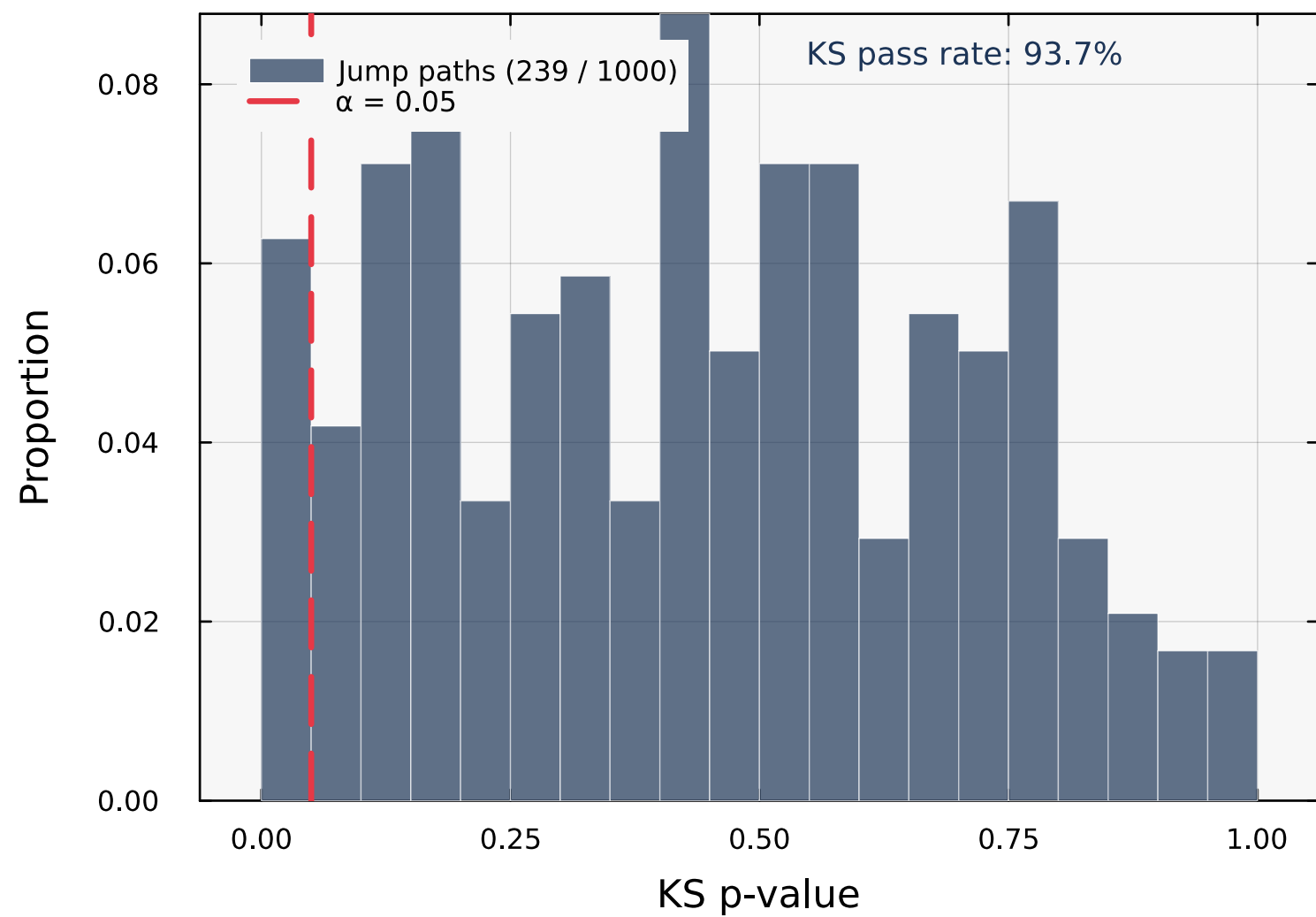
(a) In-Sample KS p-values (jump paths)
