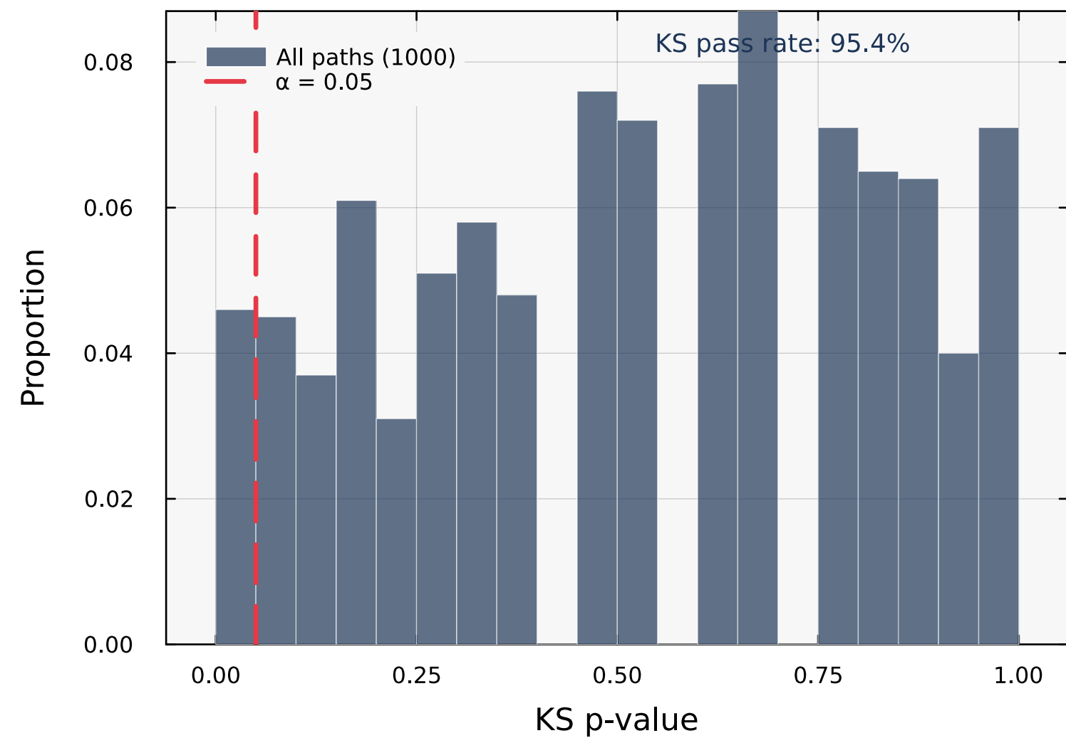
(b) Out-of-Sample KS p-values (all paths)
