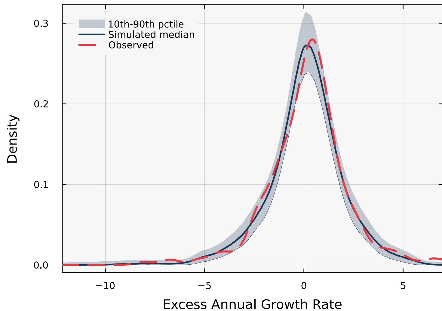
(c) OoS Density Fan Chart (all paths)
