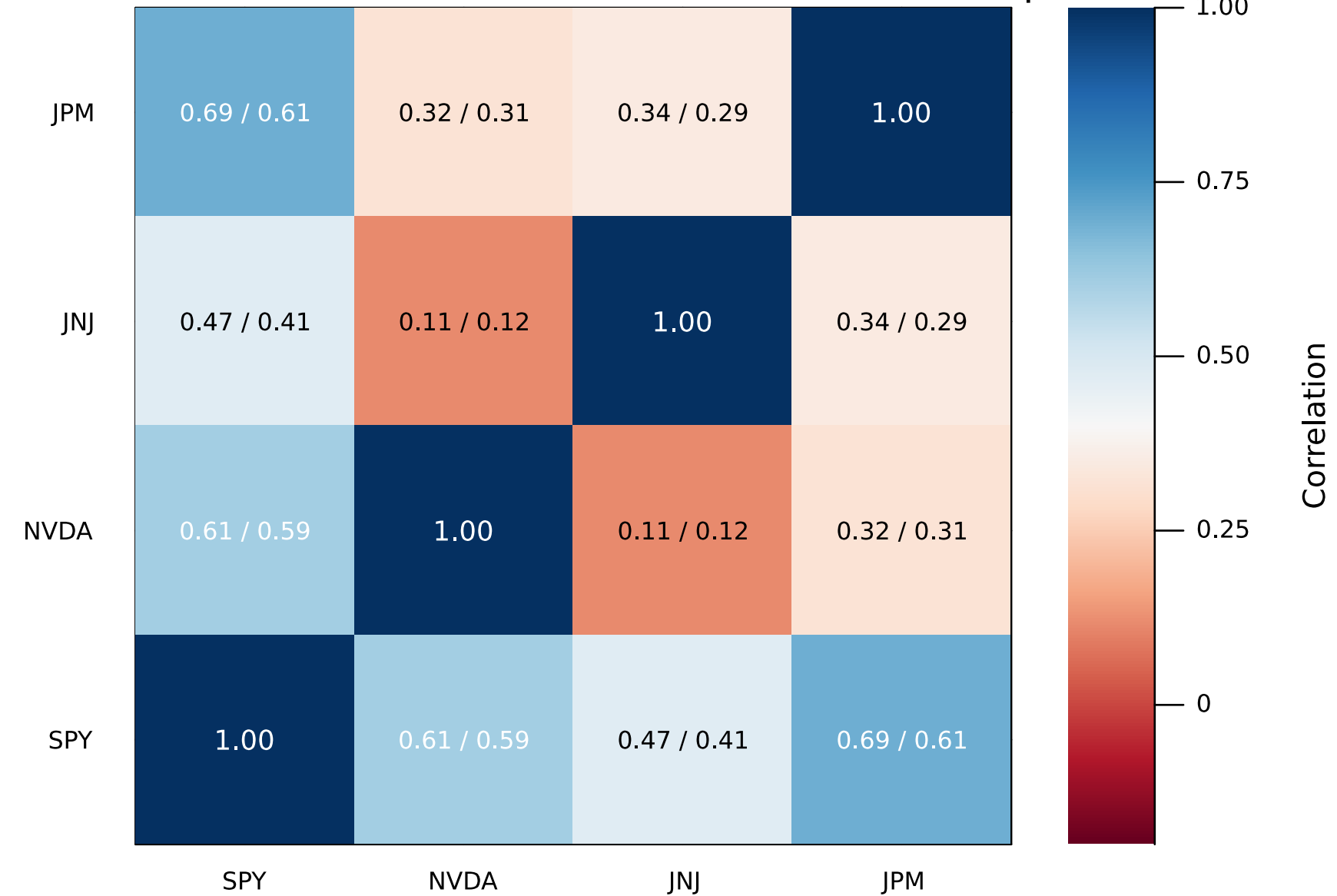
(b) Pairwise Correlations: Observed / Student-t Copula
