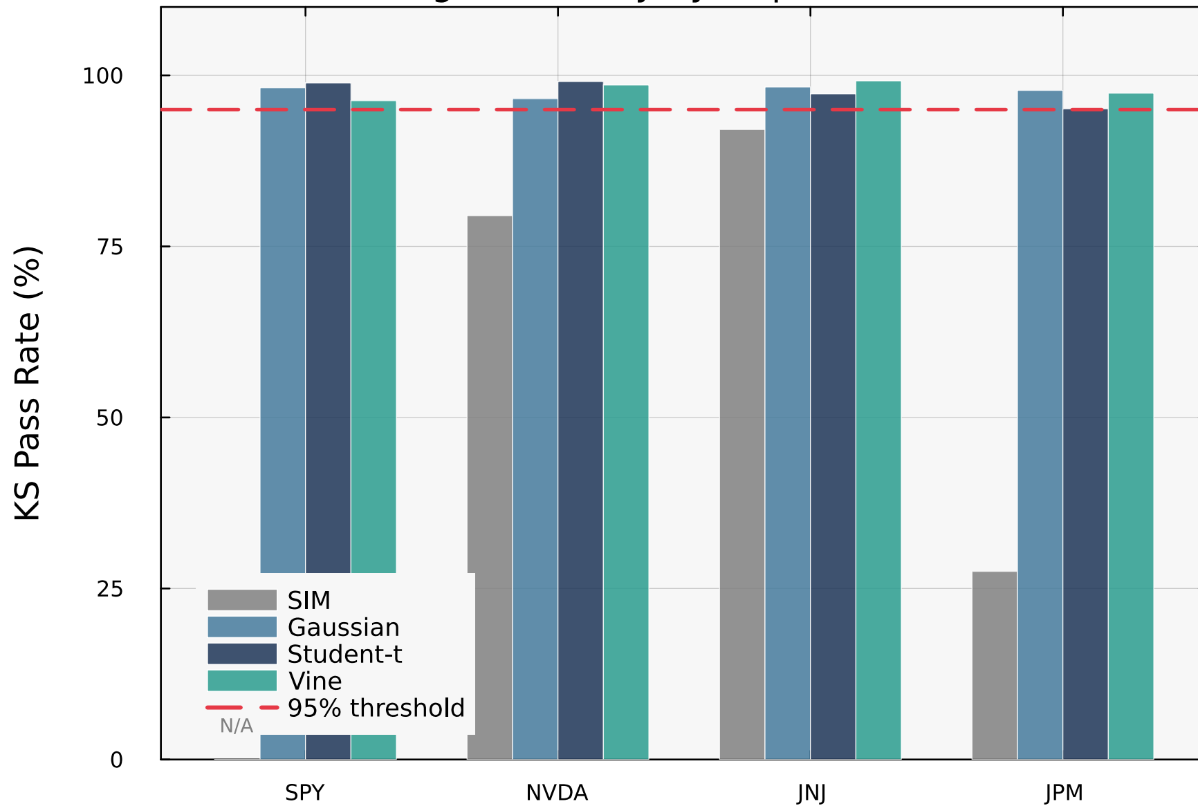
(a) Marginal Fidelity by Dependence Model
